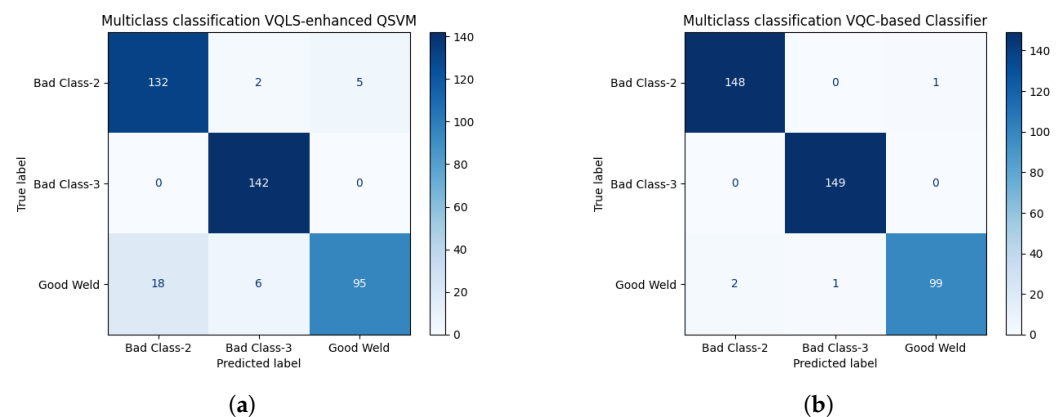
Figure 11. Confusion matrices for multiclass (3-class) classification at feature size 63: (a) VQLS-enhanced QSVM; (b) VQC-based classifier.
