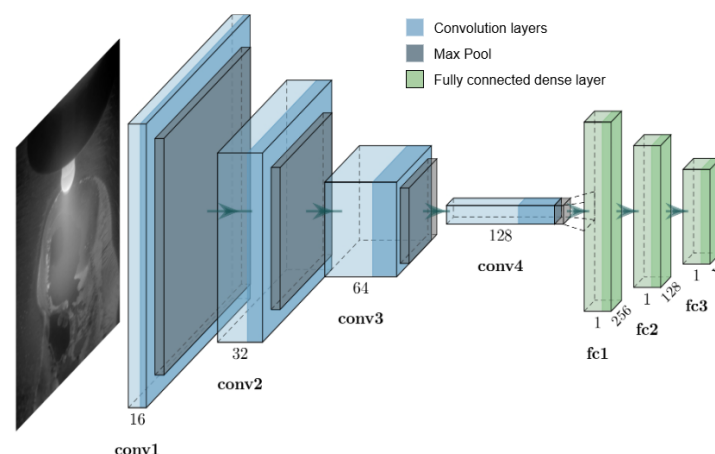
Figure 2. CNN architecture for feature extraction. The last fully connected layer outputs a feature vector X \in \{7, 15, 31, 63, 127\} .
