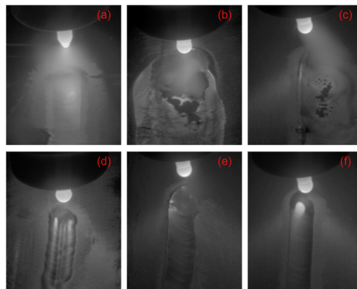
Figure 7. Six-class categorization of welding defects: (a) good weld, (b) burn through, (c) contamination, (d) lack of fusion, (e) misalignment, and (f) lack of penetration. These images are taken from Kaggle [20].
