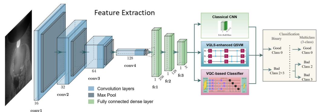
Figure 1. Full architecture of the study, showing CNN-based feature extraction followed by three classification approaches: classical CNN, VQLS-enhanced QSVM, and VQC-based classifier.
