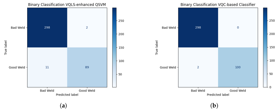
Figure 10. Confusion matrices for binary classification at feature size 63: (a) VQLS-enhanced QSVM; (b) VQC-based classifier.
