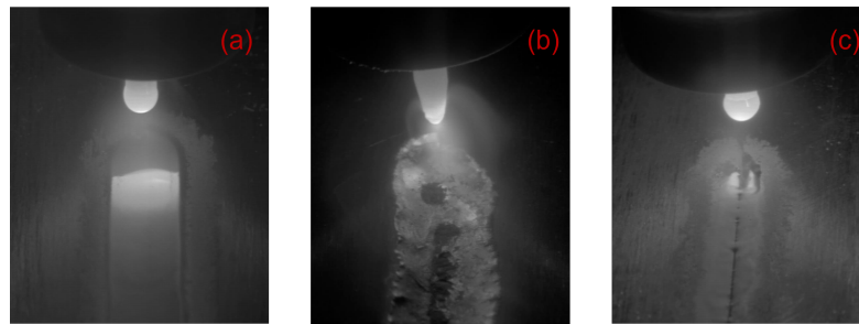
Figure 8. Three-class categorization of welding defects: (a) good weld, (b) contamination, and (c) lack of fusion.
