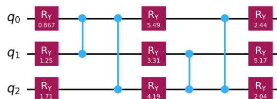
Figure 5. Quantum circuit for hardware-efficient ansatz.
