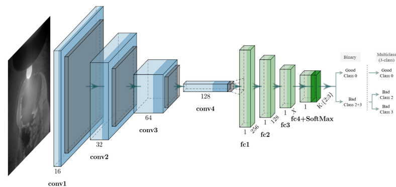
Figure 3. Classical CNN architecture for classification.
