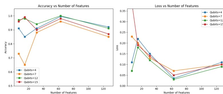
Figure 9. Hyperparameter tuning for the VQC-based classifier over feature sizes (7, 15, 31, 63, 127) and qubit configurations (4, 7, 12, 15), with a fixed batch size of 16.
