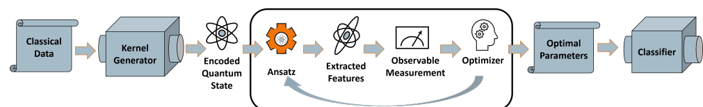
Figure 4. Pipeline for VQLS-enhanced QSVM algorithm.
