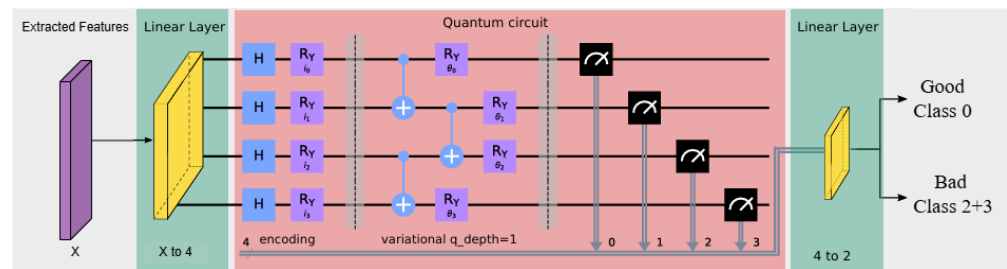
Figure 6. Pipeline for VQC-based classifier algorithm for binary classification.
