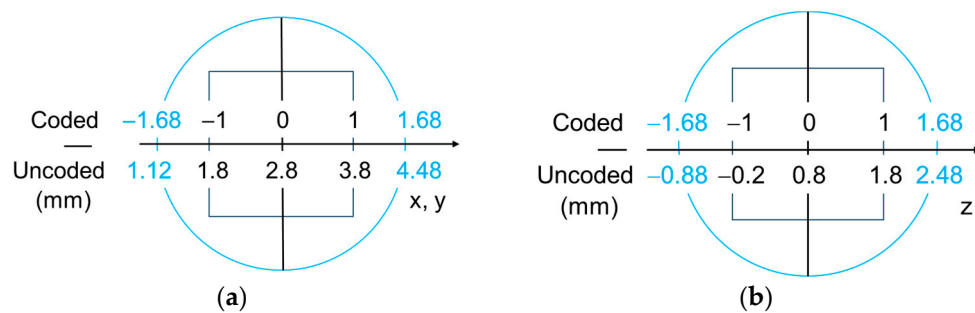
Figure 1. Coded and actual values of the ICP torch position on the x-, y-, and z-axes used for BBD (a) and CCD optimisation (b). The blue values indicate the values for the star points of CCD. These were rounded to decimal places during experiments, since the torch position could be adjusted in increments of 0.1 mm.
