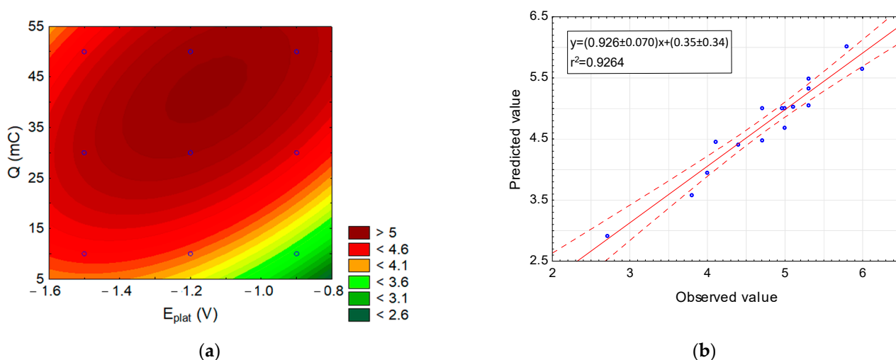
Figure 3. (a) CCD–CSP response surface profile of the germanium peak current versus charge and plating potential generated after optimisation of the bismuth plating parameters constructed for an optimal bismuth concentration equal to 16.7 mM. (b) Plot comparing the predictions from the design and experimental data for CCD. The 95% confidence band selected using a dashed line. The peak currents were measured for differential pulse voltammograms recorded in solutions containing 30 nm Ge(IV), 0.05 M acetate buffer (pH of 4.4), 1 mM catechol, 1 mM of V(IV), and 1.5 mM of HEDTA after accumulation at E_{acc} = 0.4\text{ V} for t_{acc} = 30\text{ s} . Bismuth plating was performed in 0.34 M \text{HClO}_4 .
