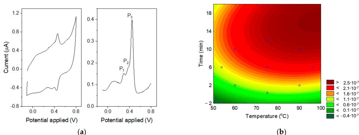
Figure 4. (a) CV and DPV voltammograms recorded in solution containing 20 times diluted Ginkgo biloba extract. (b) CCD response surface profile of P3 DPV peak current vs. time and temperature of extraction. Supporting electrolyte: 0.15 M acetic acid, E_{acc} = 0 V, t_{acc} = 5 s, 0.1 V/s (CV).
