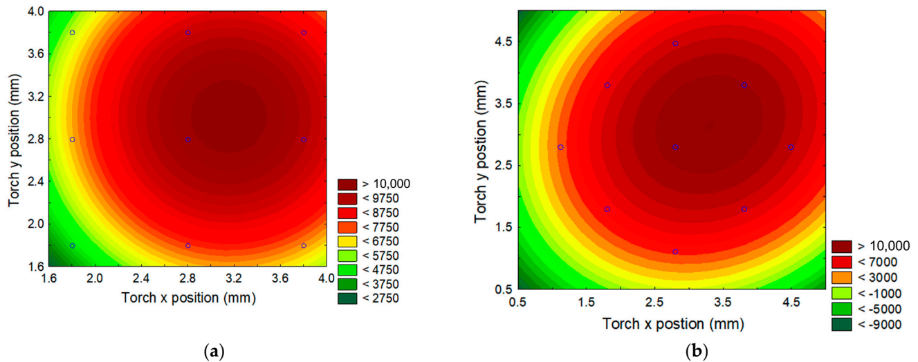
Figure 2. (a,b) Response surface profiles of the intensity of the indium signal versus the position of the ICP torch x and y generated after optimisation of the variables using (a) BBD1 and (b) CCD designs constructed for the optimal position z ( z = 0.3 mm (BBD1) or z = -0.9 mm (CCD)).
