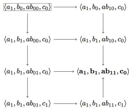
Figure 8. Transition graph of the process hitting in Figure 7 from the state represented by grayed processes.
