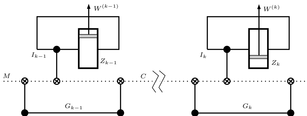
Figure 4. Representation of the M qubit processing by consecutive cylinders. First, a CNOT is applied, controlled by the local security qubit G_k . It unlocks the M qubit, so that it can undergo a second CNOT, controlled by the internal qubit I . After Z_k has finished its cycle, a new CNOT, again controlled by G_k prepares M for the transmission to Z_{k+1} .
