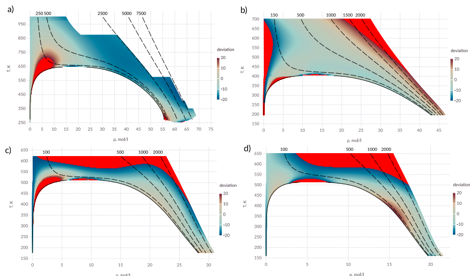
Figure 4. Percentage deviation in thermal conductivity coefficient in the T – \rho diagram; (a) water; (b) ammonia; (c) methanol; (d) ethanol; points in which the deviation exceeds 20% are shown in red; solid lines—saturation line; dashed lines—isothers, pressure is indicated above the lines in bars.
