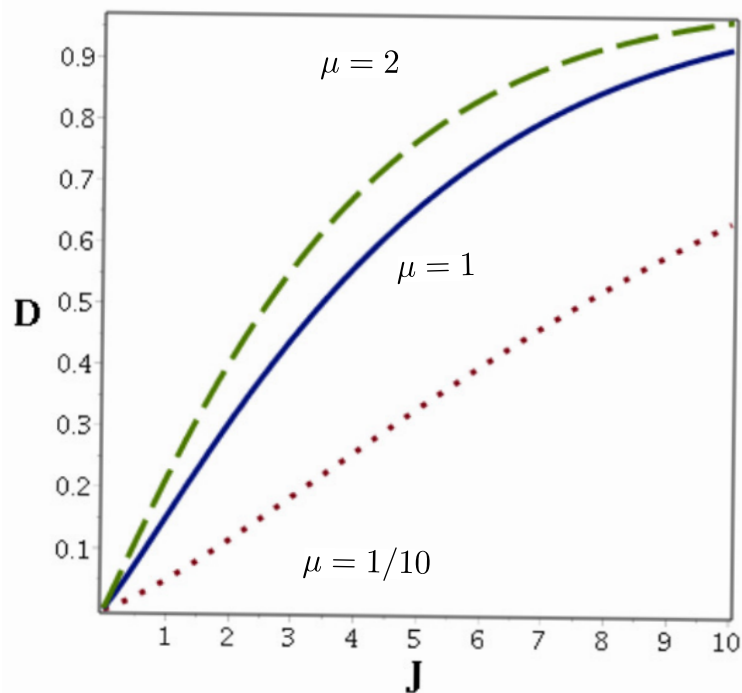
Figure 1. Trace distance between the Gazeau–Kluder coherent states |J, 0\rangle given by Equation (3) and the Perelomov coherent states |z = \sqrt{J}\rangle depicted for selected values of the rescaled susceptibility \mu .
