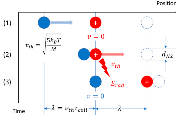
Figure 7. Molecule–ion interaction inside a gas of temperature T leading to an exchange of motional energy between the molecule and ion and causing the emission of a pulse of electromagnetic radiation upon interaction (2).
