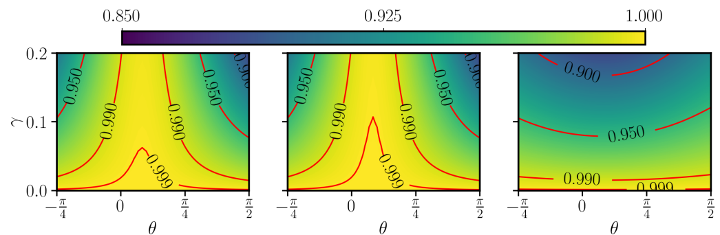
Figure 4. Zoom into the high fidelity region ( \mathcal{F}_1 > 0.85 ) for the data in Figure 3. We see that the hierarchy established in Figure 3 between the three sweep functions is maintained.
