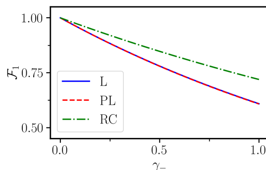
Figure 5. Final fidelity at the end of the different STA control protocol as a function of the decay rate \gamma_- for a jump operator \hat{\sigma}_- , of the three sweep functions linear (blue solid line), polynomial (dashed red line) and Roland–Cerf (green dashed-dotted line). It can be seen that the linear and the polynomial control protocol have the same behavior because of the very similar occupation time of the state |1\rangle . On the contrary, with the Roland–Cerf, the population of state |1\rangle is occupied later than the other two, and therefore it is more robust. The other simulation parameters are the same as in Figure 1.
