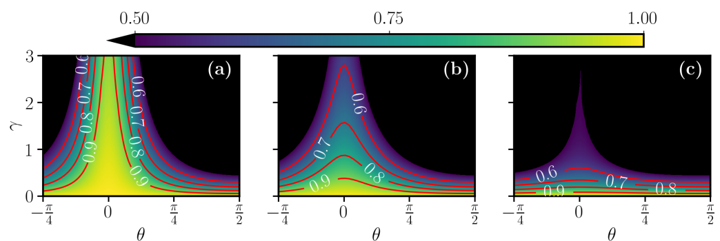
Figure 7. Final fidelity of Equation (14) at the end of the different STA control protocols, (a) linear, (b) polynomial, and (c) Roland–Cerf, as a function of \theta and the common rate \gamma . In contrast with the one-qubit case, the linear and the polynomial protocols behave differently because of their different temporal profile of the fidelity, as shown in Figure 6c. In this case, the linear is more robust than the other two around \theta = 0 . The other simulation parameters are the same as in Figure 6.
