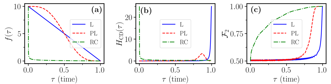
Figure 6. Temporal profile for the two-qubit case of (a) the same three sweep functions of Section 2.1; (b) the coefficients of the matrix elements in Equation (16) of the counterdiabatic term, for the three sweep functions; (c) the fidelity \mathcal{F}_2 of Equation (14), in the absence of any error and dissipation ( \gamma = 0 ). The simulation parameters are \omega_{g1} = 30 , T = 10 , \alpha_g = 10 , f_0 = 10 , \gamma = 0 .
