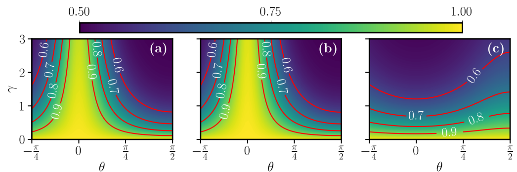
Figure 3. Color map of the final fidelity of Equation (11) at the end of the control protocols for the STA corresponding to f_L(\tau) in (a), f_{PL}(\tau) in (b), f_{RC}(\tau) in (c) for the jump operator of the Equation (12) as a function of \theta and of the decay rate \gamma . The first two control protocols are very stable around \theta = 0 and also in this case, (a,b) look very similar for the same reason explained in Figure 2. Panel (c), instead, presents the opposite behavior, with respect to (a,b), being more robust around \theta = \pi/2 . The other simulation parameters are the same as in Figure 1.
