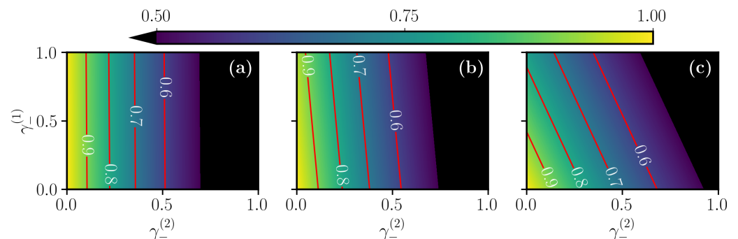
Figure 8. Final fidelity at the end of the different STA protocols, (a) linear, (b) polynomial and (c) Roland–Cerf, as a function of the two different local decay rates of the two qubits. The other simulation parameters are the same as in Figure 6.
