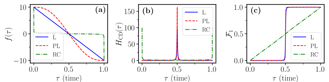
Figure 1. Time dependence, for the one-qubit case, of (a) the three sweep functions in Section 2.1; (b) the matrix elements of the counterdiabatic term corresponding to the three sweep functions; (c) the fidelity \mathcal{F}_1 of Equation (11) for the three sweep functions in the absence of any error and dissipation ( \gamma = 0 ). Parameters used for all the simulations are T = 10, \alpha_g = 10, f_0 = 10 , in the dimensionless units introduced just before Equation (9).
