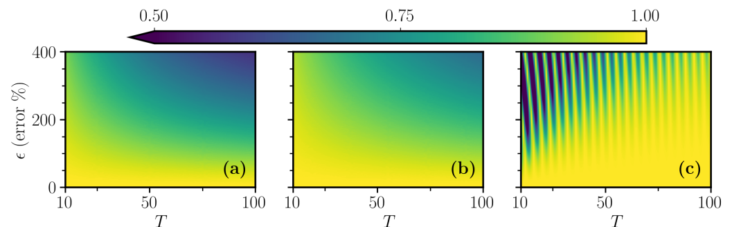
Figure 2. Final fidelity \mathcal{F}_1 of the three sweep functions (a) linear, (b) polynomial and (c) Roland–Cerf, in the presence of the indicated error \epsilon . The behavior of (a) is very similar to that of (b) because the two corresponding control protocols, linear and polynomial, have a very similar fidelity temporal shape, as observed in Figure 1c, while, in the Roland–Cerf protocol, we see characteristic oscillations [35]. These are related to accidental cancellations of higher-order non-adiabatic processes that lead to an accidentally increased performance. The other simulation parameters are the same as in Figure 1.
