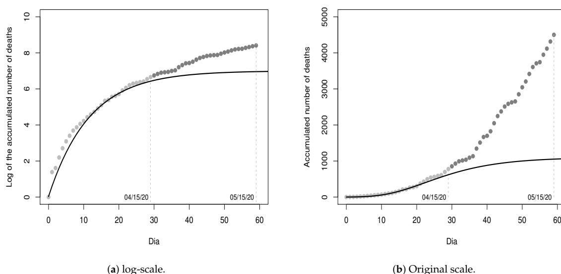
Figure 4. Data from 17 March 2020 to 15 May 2020 and fitted model \hat{Y}_t^{(1)} , for t \geq 0 .
