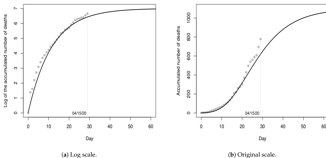
Figure 3. Data from 17 March 2020 to 15 April 2020 and fitted model \hat{Y}_t^{(1)} , for t \geq 0 .
