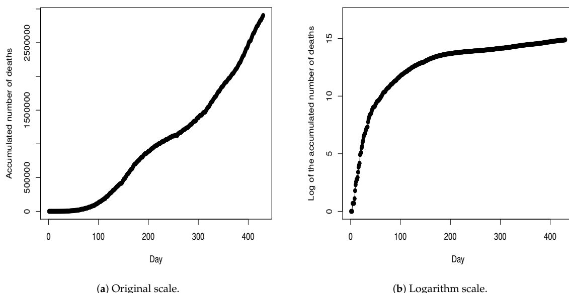
Figure 2. Cumulative number of deaths until day t , for t = 0, 1, \dots, n .
