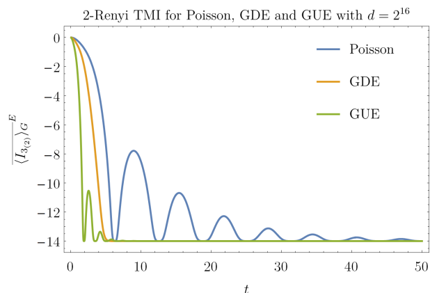
Figure 3. Plot of the upper bound for \overline{\langle I_{3(2)}(t) \rangle_G}^E , see r.h.s of Equation (27), for E \equiv P , E \equiv \text{GUE} and E \equiv \text{GDE} with d_C = d_D = d^{1/2} and d = 2^{16} . GUE and Poisson reveal oscillations before the plateau whose amplitude and damp time increases with the system size d , see Equations (29) and (30), respectively. For GDE there are no oscillations: the plateau is reached in O(\sqrt{\log d}) .
