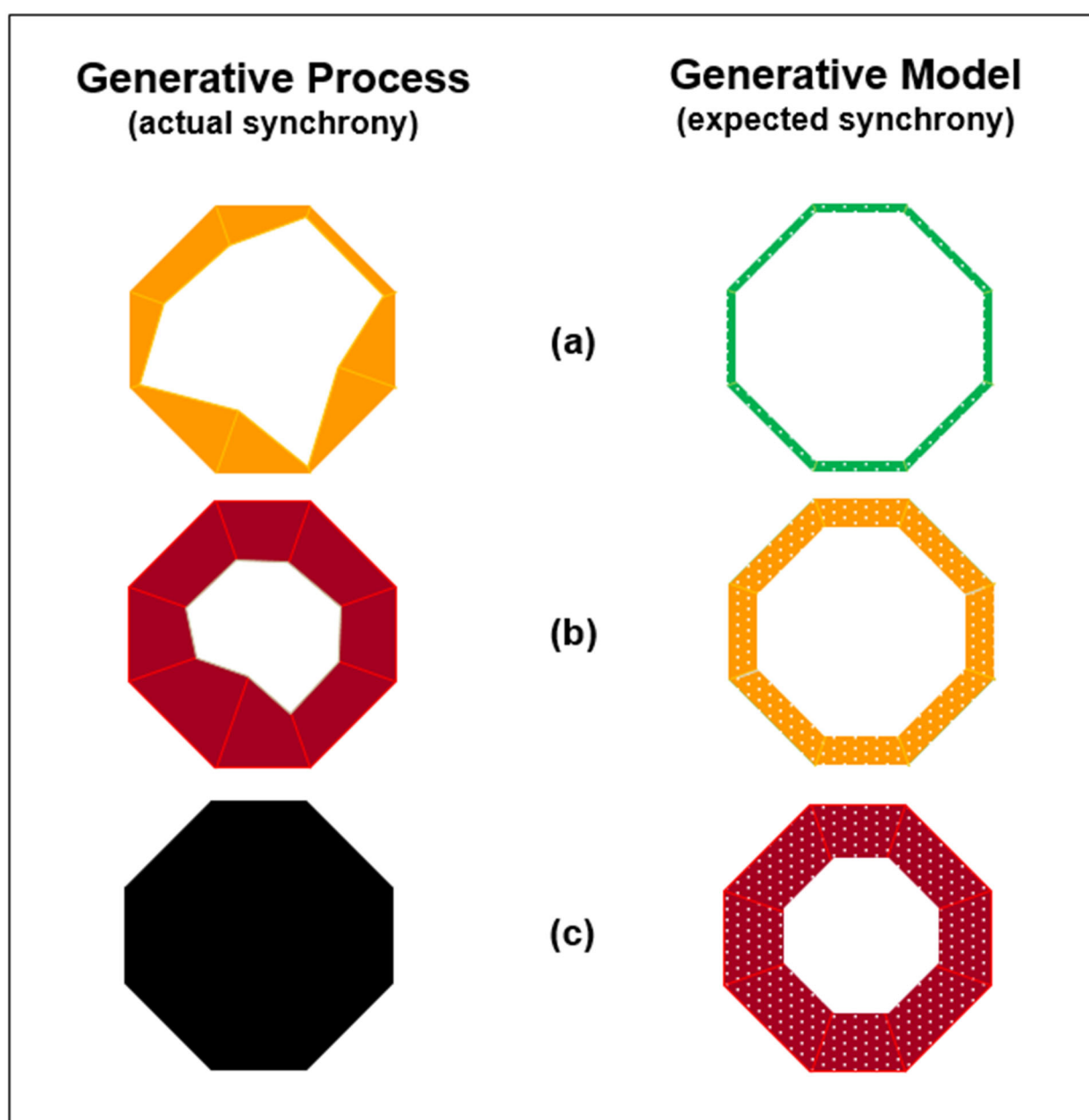
Figure 3. Expected synchrony versus actual synchrony. (a) Expected survival information deficit in generative model is minimal but actual survival information deficit in generative process is medium. (b) Agent updates expected survival information deficit to medium, but the actual survival information deficit is high. (c) Agent updates expected survival information deficit to high, but the actual survival information deficit is too high for the agent to survive.
