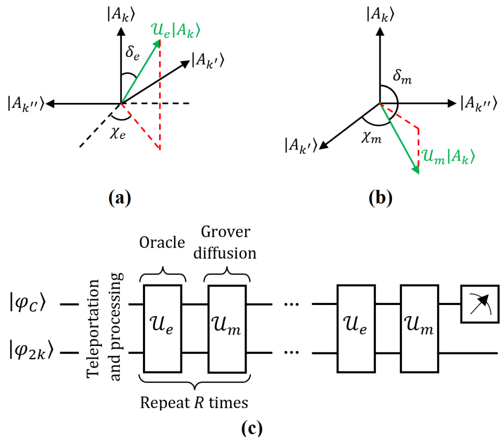
Figure 11. (a) Effect of U_e on each |A_k\rangle , k \in K as a multidimensional rotation by angles \delta_e and \chi_e with respect to itself and other |A_{k'}\rangle , k' \in K . (b) Effect of U_m on each |A_k\rangle as a multidimensional rotation by angles \delta_m and \chi_m with respect to itself and other |A_{k'}\rangle . (c) Simplified Grover circuit considering the oracle U_e and the Grover diffusion operator U_m , both repeated R times after teleportation and processing, with a possible control state measurement at the end.
