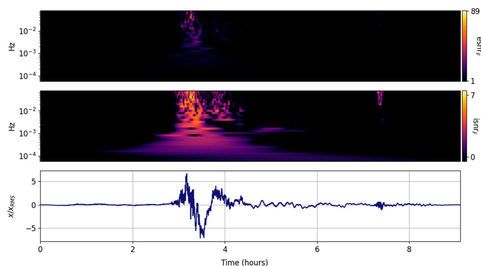
Figure 9. Scaled input signal (lower panel) and its STX information snr ( isnr_{F,m,n} , middle panel) and entropy snr ( esnr_{F,m,n} , upper panel) per frequency band.
