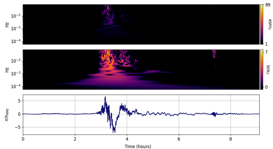
Figure 6. Scaled input signal ( lower panel ) and its CWT information snr ( isnr_{F,m,n} , middle panel ) and entropy snr ( esnr_{F,m,n} , upper panel ) per frequency band.
