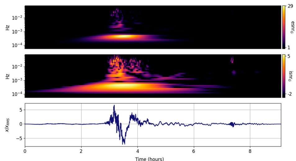
Figure 8. Input signal ( lower panel ) and its STX grid information snr ( isnr_{G,m,n} , middle panel ) and entropy snr ( esnr_{G,m,n} , upper panel ).
