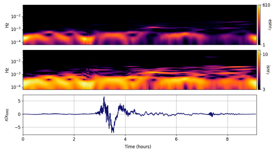
Figure 4. Scaled input signal ( lower panel ) and its GTX information snr ( isnr_{T,m,n} , middle panel ) and entropy snr ( esnr_{T,m,n} , upper panel ) per time step.
