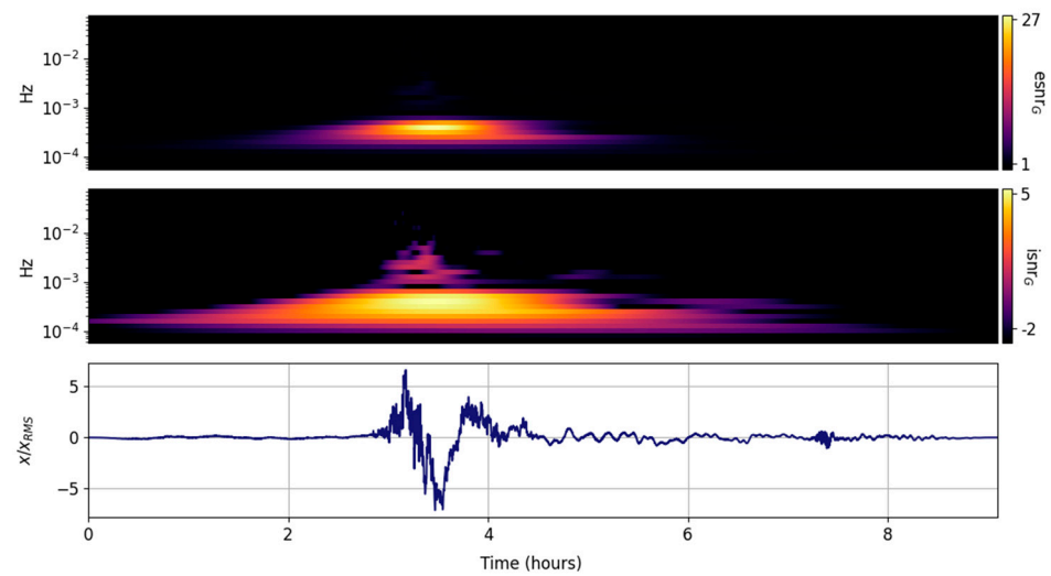
Figure 5. Input signal ( lower panel ) and its CWT grid information snr ( isnr_{G,m,n} , middle panel ) and entropy snr ( esnr_{G,m,n} , upper panel ).
