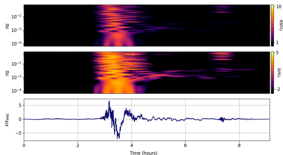
Figure 3. Scaled input signal ( lower panel ) and its GTX information snr ( isnr_{F,m,n} , middle panel ) and entropy snr ( esnr_{F,m,n} , upper panel ) per frequency band.
