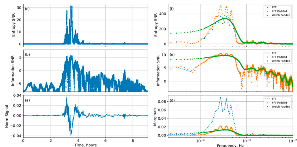
Figure 1. Time (a–c) and frequency (d–f) representations of the signal observed by an IMS infrasound station in New Caledonia. The solid blue line represents the FFT of the input signal, the orange dots represent the FFT of the zero-padded signal, and the green line the Welch periodogram of the zero-padded STFT subwindow with a high overlap.
