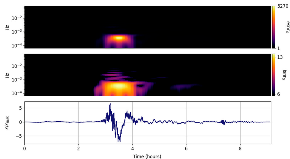
Figure 2. Input signal ( lower panel ) scaled by its rms and its GTX grid information snr ( isnr_{G,m,n} , middle panel ) and entropy snr ( esnr_{G,m,n} , upper panel ).
