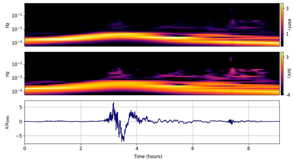
Figure 7. Scaled input signal ( lower panel ) and its CWT information snr ( isnr_{T,m,n} , middle panel ) and entropy snr ( esnr_{T,m,n} , upper panel ) per time step.
