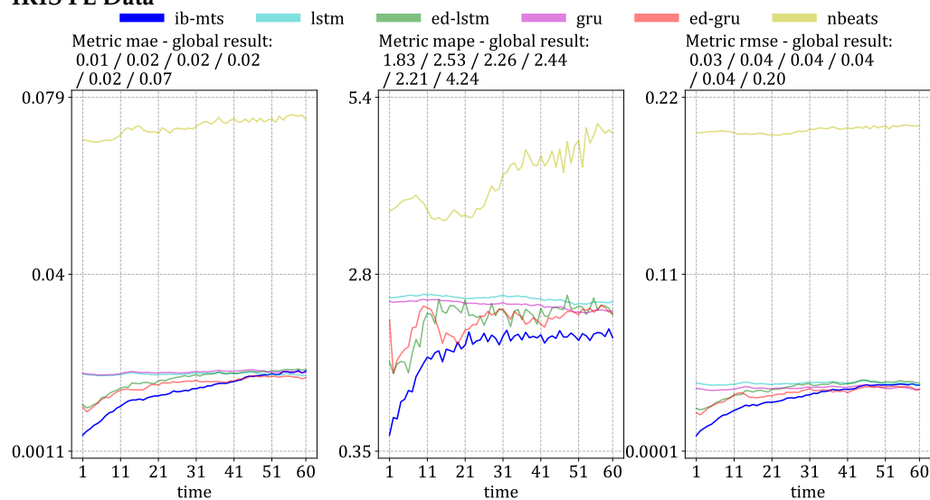
Figure A1. Detailed MTS metrics evaluation on the test set for the direct prediction setup. The evaluations are given for each solar activity: the first row of results is for QS activity, the second row is for AR, and the last row is for FL.
