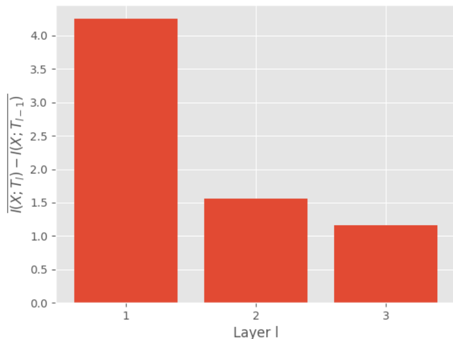
Figure A4. Mean difference in MI of subsequent layers l and l + 1 . Positive numbers indicate compliance with the DPI. MI was measured on the MNIST training using the EDGE MI estimator on a simple MLP [4].
