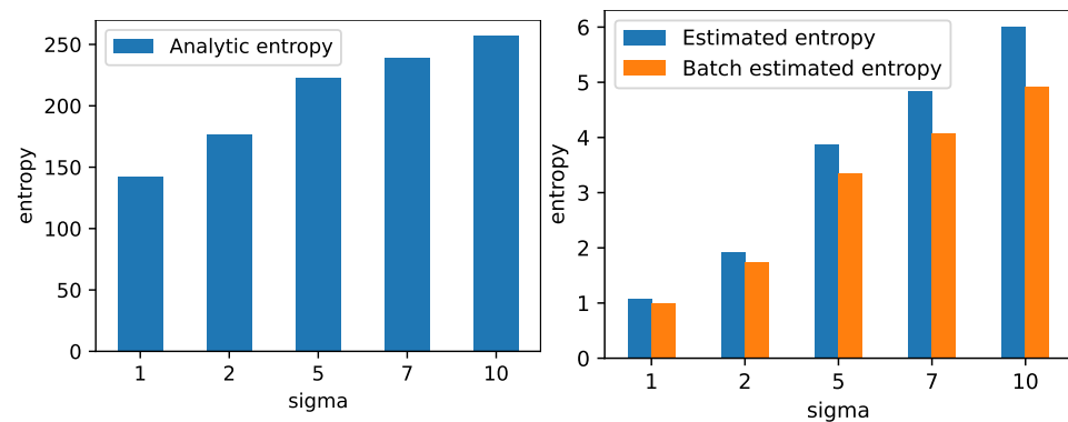
Figure 2. The leftmost plot shows the entropy calculated using Equation (14) of a 100-dimensional normal distribution with zero mean and an isotropic covariance matrix for different variances. The variances are given along the x-axis. The rightmost plot shows the entropy estimated using Equation (1) for the same distribution. The plots illustrated that the analytically computed entropy and the estimated quantity follow the same trend.
