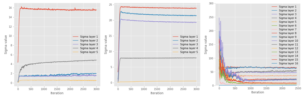
Figure 8. Evolution of kernel width as a function of iteration for the three networks that we considered in this work. From left to right, plots show the kernel width for the MLP, CNN, and VGG16. The plots demonstrate how the optimal kernel width quickly stabilizes and stays relatively stable throughout the training.
