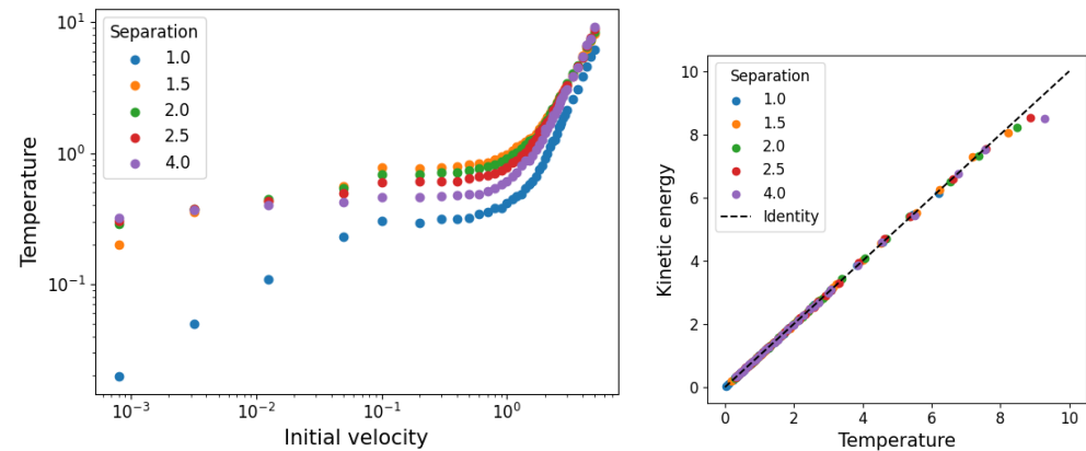
Figure 4. On the left: fitted temperature in equilibrium as a function of the initial velocity range V_M for different initial separations. On the right: agreement between fitted temperature and the average kinetic energy.
