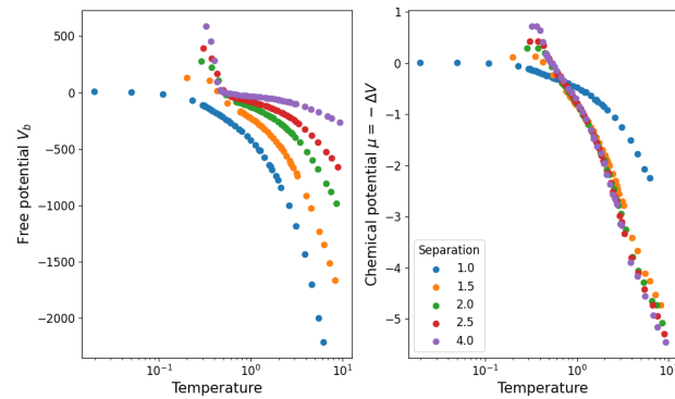
Figure 11. Partition function parameters calculated from the measured average potential energy and average number of links in the system.
