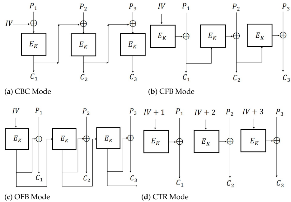
Figure 1. Encryption modes ( m = 3 ).
