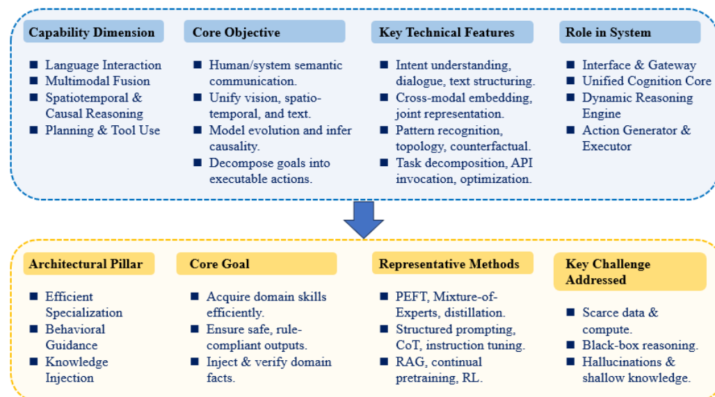
Figure 3. Core Capabilities for LLM-Enabled Traffic Systems and Key Architectural Adaptations of LLMs for Traffic Tasks.
