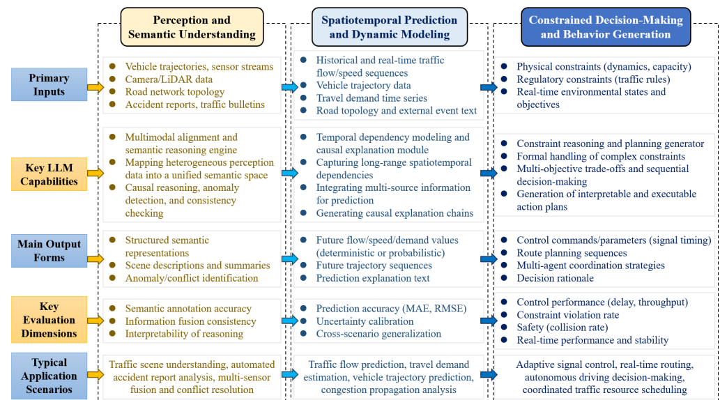
Figure 4. Core Dimensions, Capabilities, and Evaluation of LLM-Based Traffic Task Modeling.
