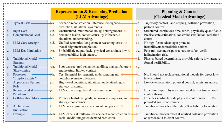
Figure 13. Comparative Analysis of LLM vs. Traditional Model Capabilities Across Transportation Task Levels. The yellow panel highlights task layers where LLMs exhibit relative advantages in representation and reasoning/prediction, while the gray panel denotes dominated by classical planning and control models. The light blue column lists comparison dimensions shared by both paradigms. Solid blue arrows indicate alignment between task attributes and the corresponding strengths or limitations of each modeling approach. Bidirectional orange arrows emphasize conceptual contrasts and information exchange between LLM-based cognitive layers and physics-based control layers. The outer blue dashed boundary represents an integrated system architecture, indicating that LLMs and traditional models are complementary components rather than substitutes. Dashed elements denote conceptual grouping instead of strict implementation boundaries.
