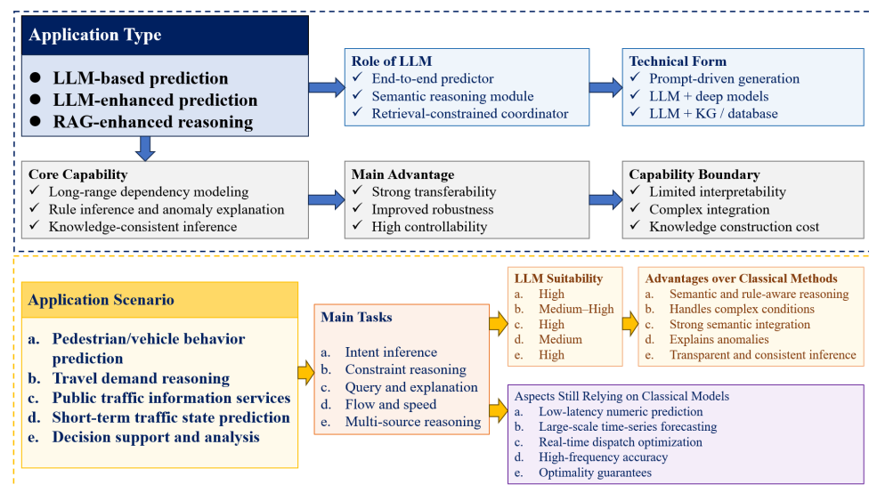
Figure 8. Application Types, System Roles, and Capability Boundaries at the Reasoning and Prediction Integration.
