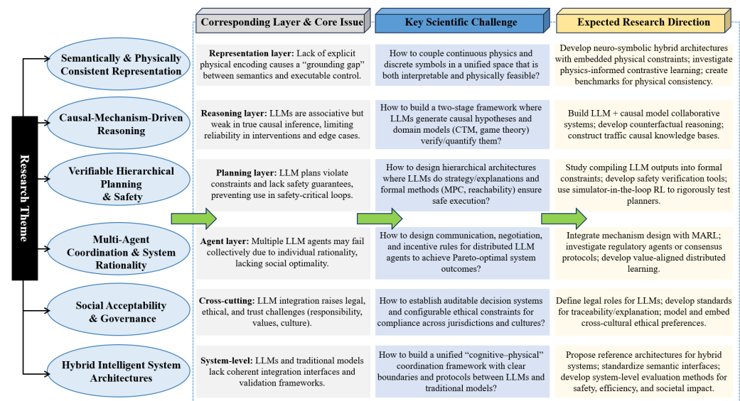
Figure 14. Future Research Agenda for LLM-Based Traffic Applications.
