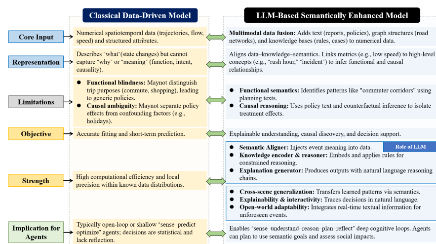
Figure 6. Comparison of Data-Driven and Semantically Enhanced Transportation Modeling.
