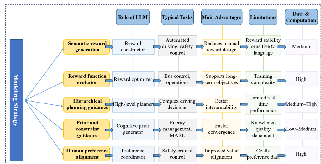
Figure 9. Modeling Strategies, Applicable Tasks, and Capability Boundaries of LLM-Guided RL.
