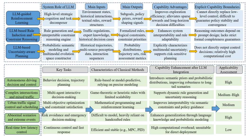
Figure 10. Application Types, System Roles, and Capability Boundaries of LLMs at Planning and Control Integration.
