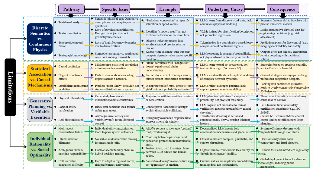
Figure 12. Capability bottlenecks and applicability boundaries of LLMs.
