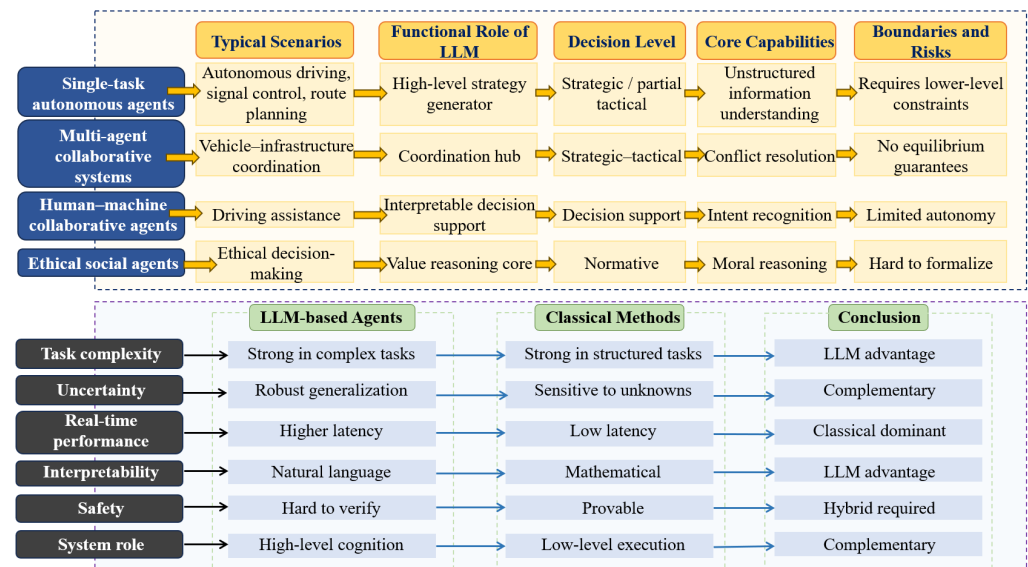
Figure 11. Scenarios, System Roles, and Capability Boundaries of LLMs at Autonomous Agent.
