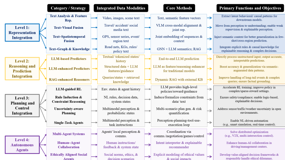
Figure 5. Four-Level LLM Integration Classification Perspective in Traffic Systems.
