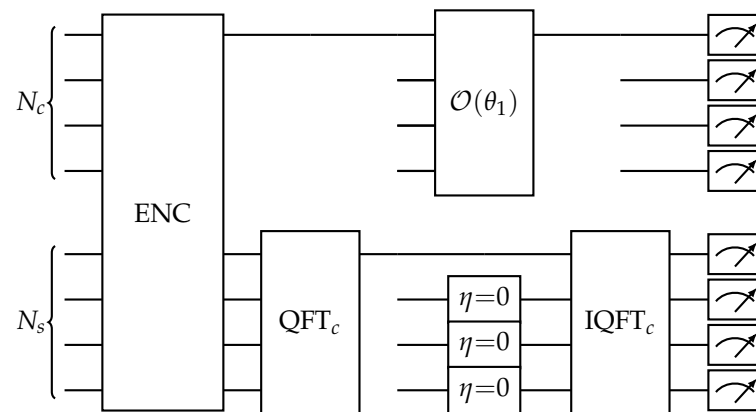
Figure 2. CV-QFNO spectral layer, branch k = 1 (1D case). The latent matrix A \in \mathbb{R}^{N_c \times N_s} is encoded via TMS-SVD into the off-diagonal covariance block \sigma_{x_{r_1} x_{r_2}} , with the n -mode upper register ( r_1 ) and the m -mode lower register ( r_2 ). A row-wise \text{QFT}_c on the lower register places \hat{A} in that block. The pyramidal interferometer O(\theta_1) is applied to the upper register; loss channels \eta = 0 are applied to all lower-register modes j \neq 1 , leaving mode k = 1 active. Each of the remaining K - 1 branches is structurally identical, with weight O(\theta_k) and mode k left free. An \text{IQFT}_c followed by homodyne measurement yields the output contribution of mode k = 1 .
