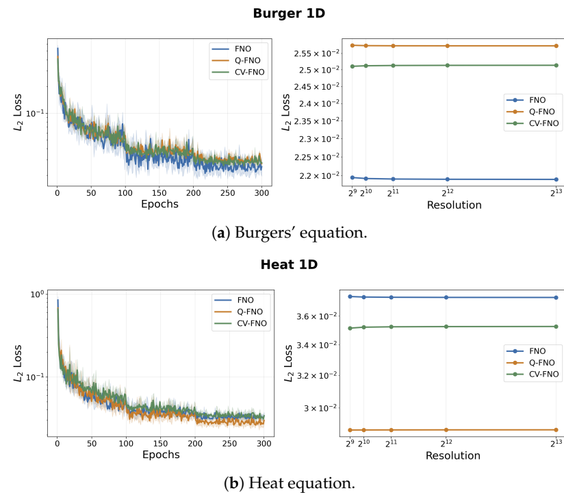
Figure 4. Training dynamics and resolution generalisation: 1D benchmarks. Left: test loss evolution over training epochs. Each solid line shows the geometric mean of the relative \ell_2 loss across four independent runs (seeds 0, 11, 22, 33); the shaded band spans \pm 1 geometric standard deviation across the seeds, reflecting run-to-run variability due to random initialisation. Right: relative \ell_2 test loss as a function of spatial resolution. The models were trained at the base resolution of 512 grid points and evaluated zero-shot at all resolutions shown, without retraining.
