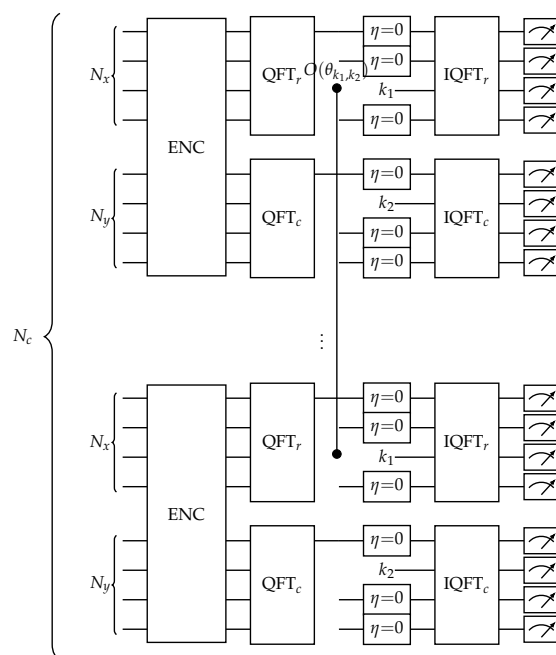
Figure 3. CV-QFNO spectral layer: mode pair (k_1, k_2) (2D case). N_c optical circuits run in parallel, one per channel l . Each circuit encodes the 2D slice A_{l,:} via TMS-SVD and applies a 2D CV-QFT on both registers. The pyramidal interferometer O(\theta_{k_1, k_2}) connects the k_1 -th upper-register wire across all N_c circuits, mixing the channel dimension for all column modes. Loss channels \eta = 0 on upper-register modes i \neq k_1 and lower-register modes j \neq k_2 then isolate the target mode pair, realising Equation (10). Homodyne measurement yields the output contribution of mode pair (k_1, k_2) .
