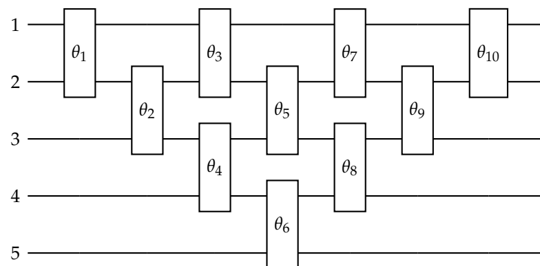
Figure 1. Pyramidal interferometer on N_c = 5 modes implementing an arbitrary 5 \times 5 orthogonal matrix in the unary subspace. Each box represents an \text{RBS}(\theta_k) gate with an independent trainable parameter \theta_k . Gates in the same column act on disjoint wire pairs and run in parallel. The circuit uses \frac{N_c(N_c-1)}{2} = 10 gates arranged in 2N_c - 3 = 7 sequential timesteps, with at most \lfloor N_c/2 \rfloor = 2 gates per timestep, achieving circuit depth O(N_c) .
