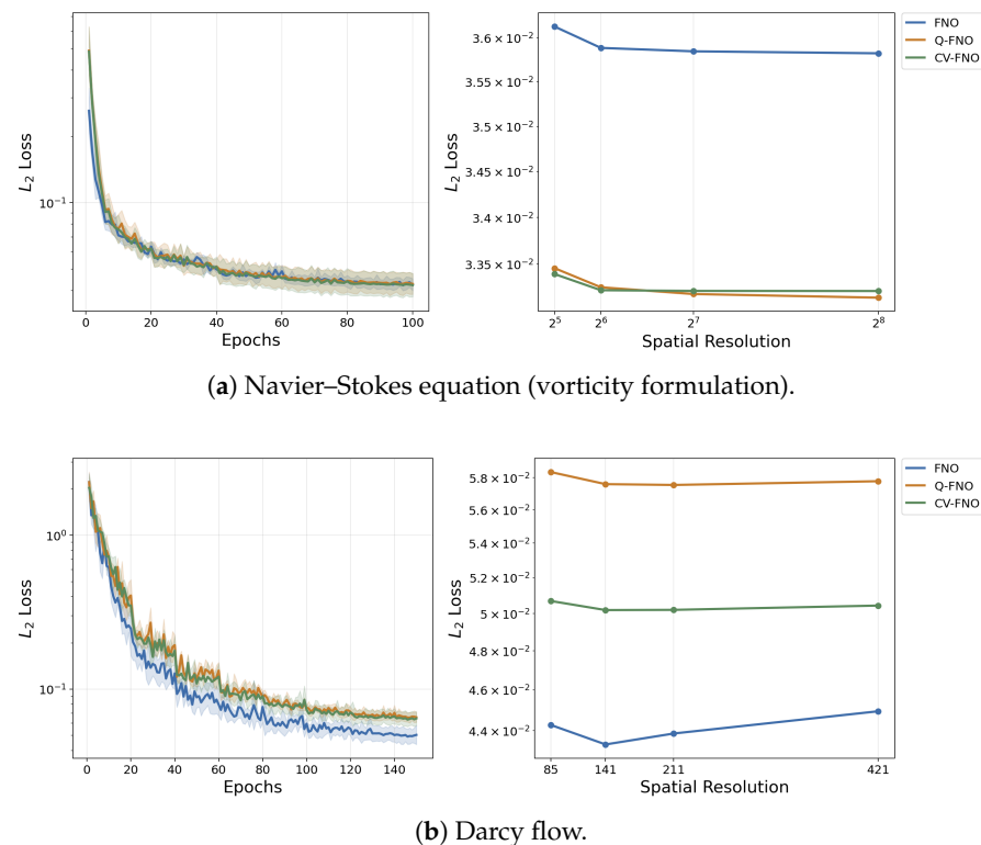
Figure 6. Training dynamics and resolution generalisation: 2D benchmarks. Left: test loss evolution over training epochs. Each solid line shows the geometric mean of the relative \ell_2 loss across four independent runs (seeds 0, 11, 22, 33); the shaded band spans \pm 1 geometric standard deviation across seeds. Right: relative \ell_2 test loss as a function of spatial resolution, evaluated zero-shot without retraining.
