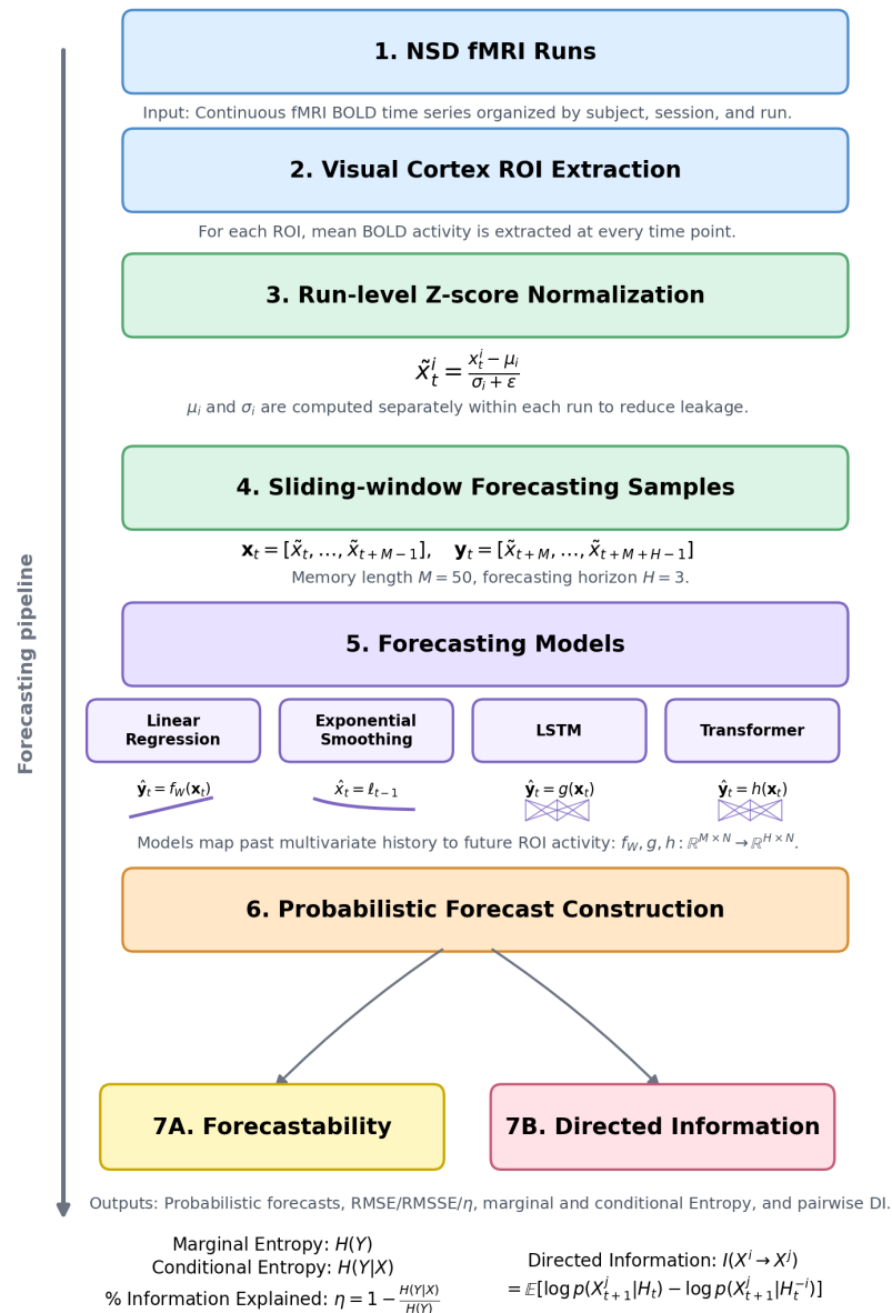
Figure 1. Overview of the proposed multivariate fMRI forecasting framework. Preprocessed BOLD time series extracted from predefined regions of interest (ROIs) were converted into sliding temporal windows and used to train forecasting models to predict future ROI activity from past observations. Forecasting performance and predictive distributions were subsequently used to compute error-based and information-theoretic measures, including conditional entropy and directed information.
