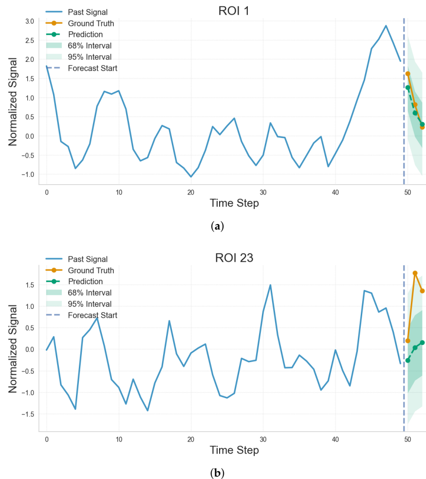
Figure 2. Illustration of probabilistic forecasting performance for two representative ROIs. The historical ROI activity preceding the forecast horizon is shown together with the ground-truth future trajectory, model prediction, and uncertainty intervals estimated from forecasting residuals. (a) Example of a well-predicted ROI trajectory, where the model accurately captures the temporal evolution of the BOLD signal within the forecast horizon. (b) Example of a poorly predicted ROI trajectory, illustrating increased forecasting error and uncertainty. These examples highlight the heterogeneous forecastability of fMRI dynamics across ROIs and temporal instances.
