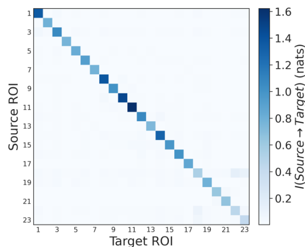
Figure 4. Directed information (DI) matrix estimated from the transformer model ( M = 50 , H = 3 ) across the selected ROIs. Larger values indicate stronger directional predictive contributions from the source ROI (rows) to the target ROI (columns). The predominantly diagonal structure suggests that short-horizon BOLD forecasting is dominated primarily by autoregressive within-ROI temporal dependencies, whereas cross-ROI directed interactions remain comparatively weaker.
