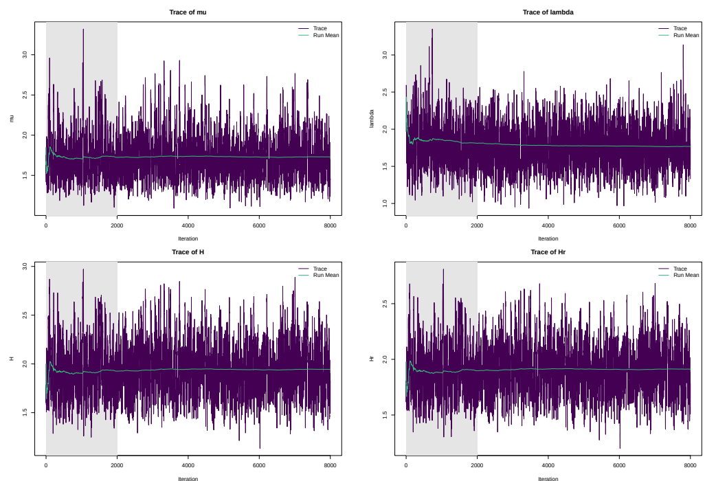
Figure 5. IG MCMC diagnostics grid n50 m40 R1.
