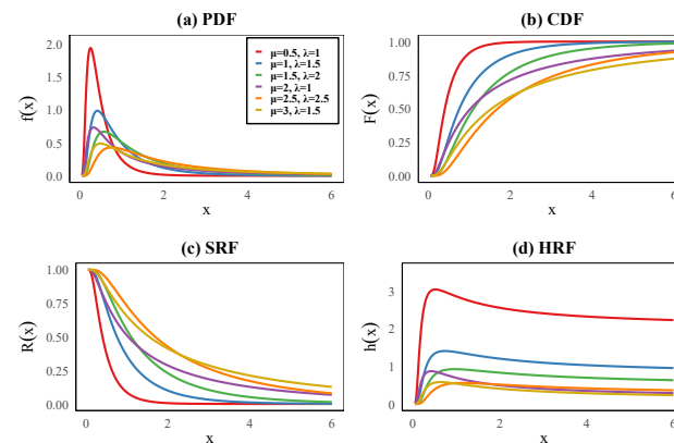
Figure 1. Inverse Gaussian: (a) probability density function (PDF), (b) cumulative density function (CDF), (c) survival function (SRF), (d) hazard rate function (HRF).
