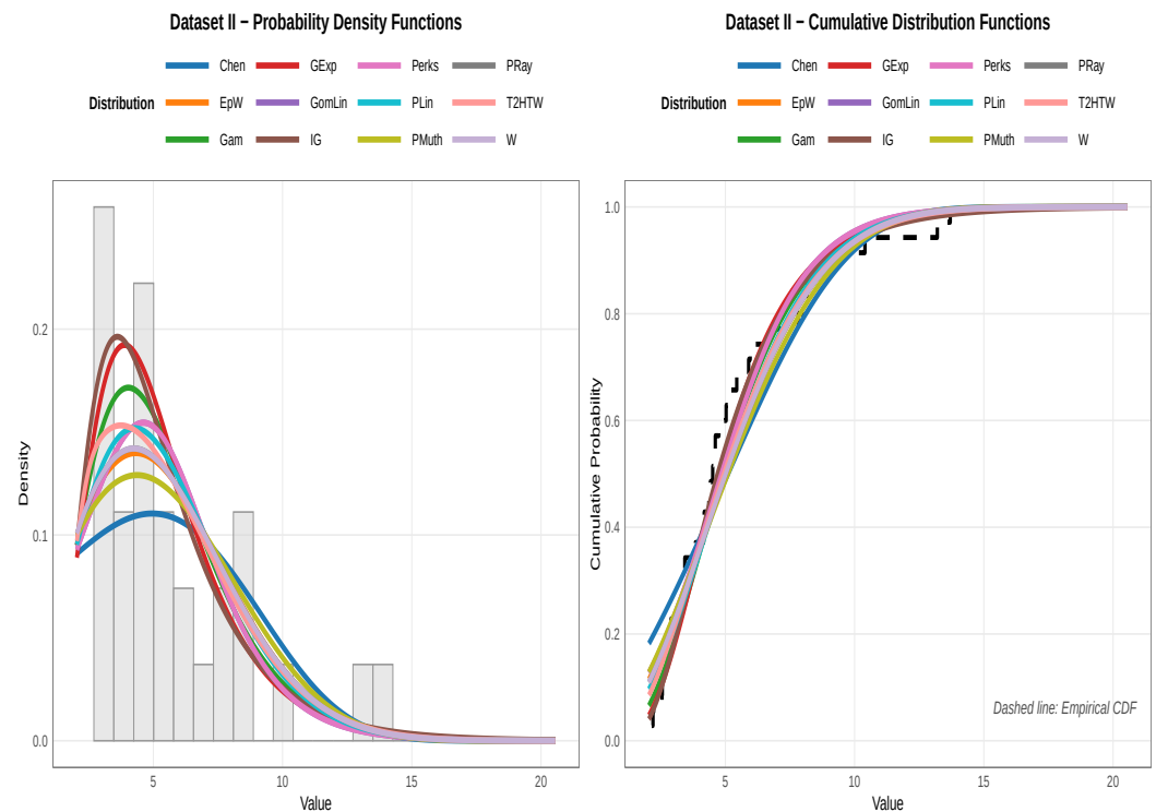
Figure 10. Fitted probability distributions for Dataset II.
