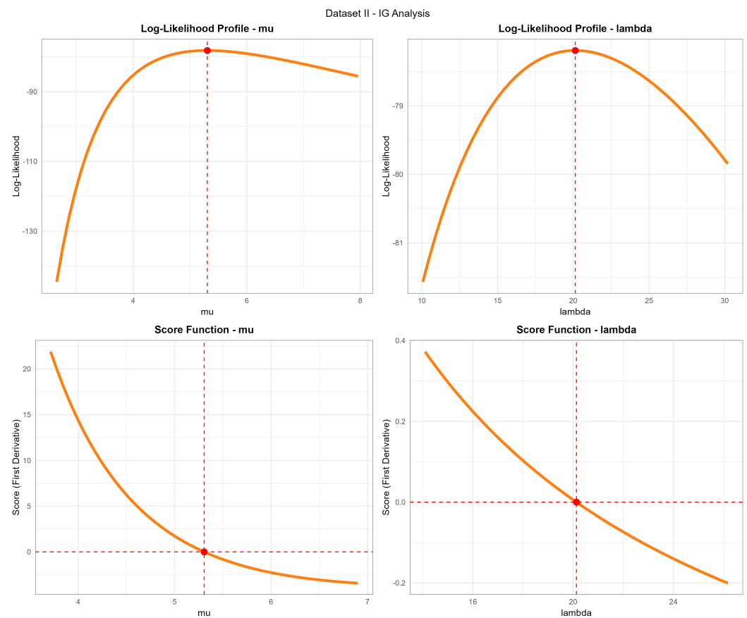
Figure 11. Inverse Gaussian distribution diagnostics for Dataset II: log-likelihood profiles and score functions for both parameters.
