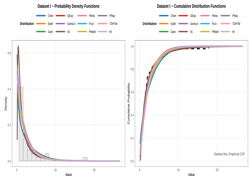
Figure 6. Fitted probability distributions for Dataset I.
