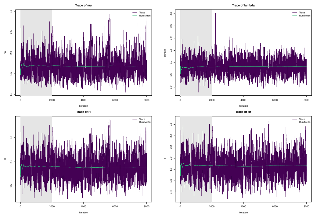
Figure 3. IG MCMC diagnostics grid.
