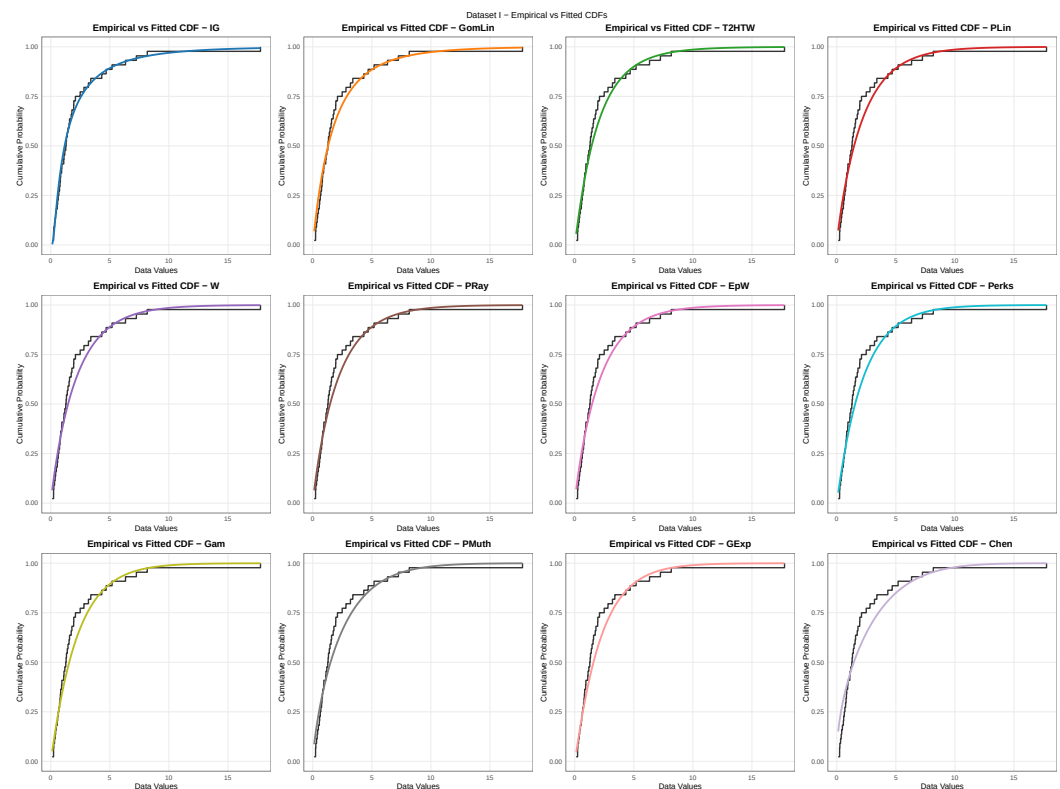
Figure 9. Empirical versus fitted CDF plots for Dataset I under fitted candidate models.
