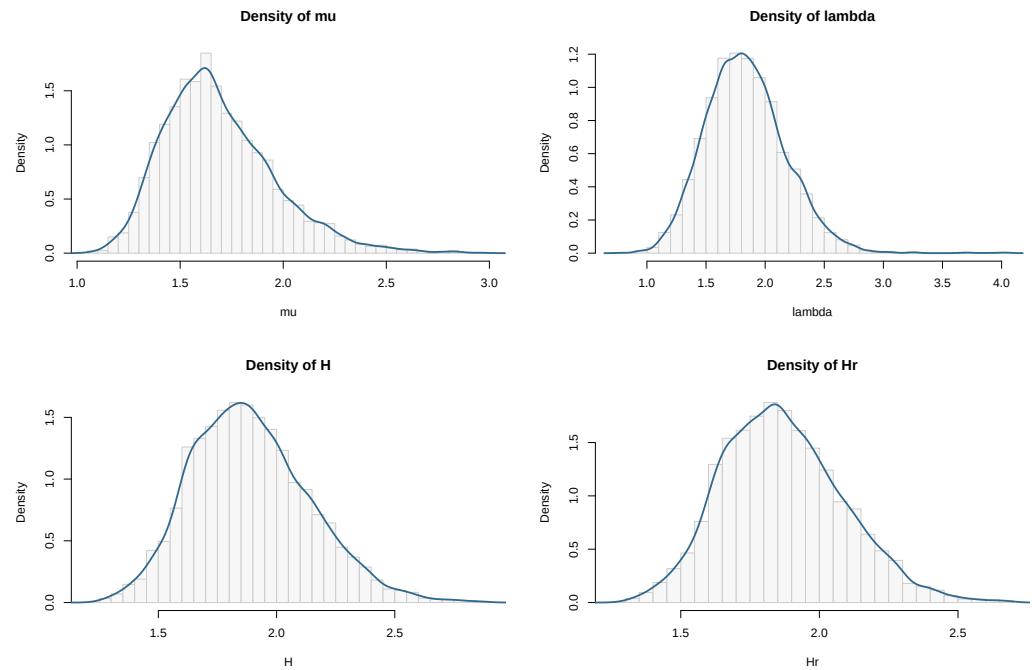
Figure 2. IG MCMC diagnostics density.
