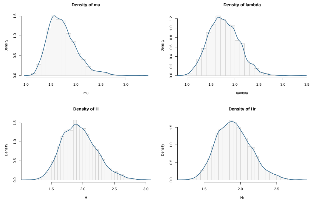
Figure 4. IG MCMC diagnostics density n50 m40 R1.
