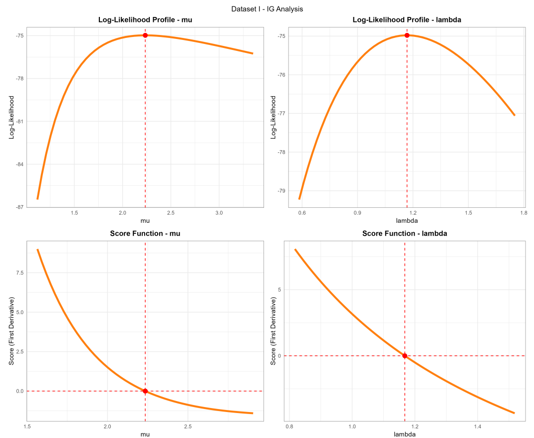
Figure 7. Inverse Gaussian distribution diagnostics for Dataset I: log-likelihood profiles and score functions for both parameters.
