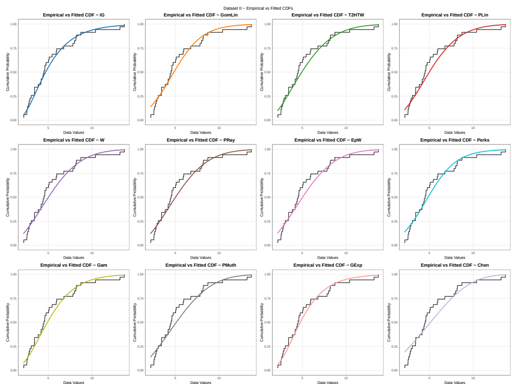
Figure 13. Empirical versus fitted CDF plots for Dataset II under fitted candidate models.
