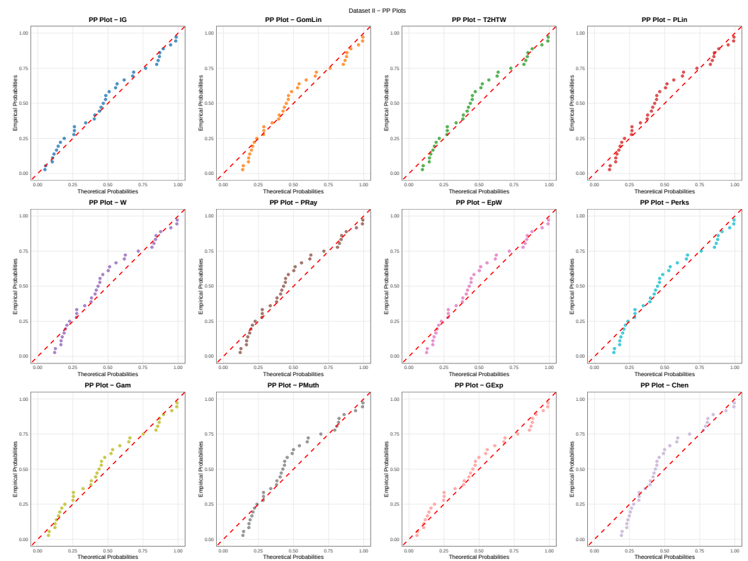
Figure 12. Probability–Probability (PP) plots for Dataset II under fitted candidate models.
