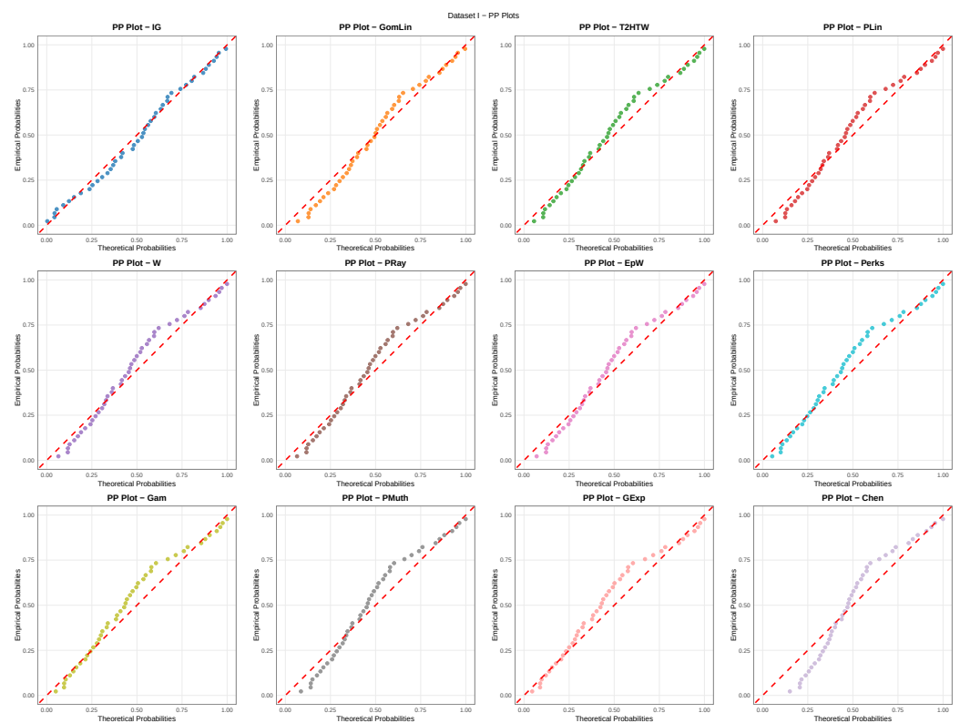
Figure 8. Probability–Probability (PP) plots for Dataset I under fitted candidate models.
