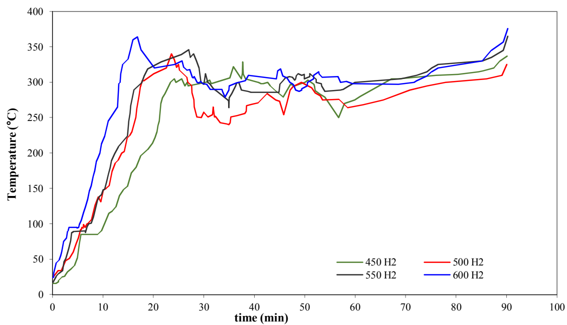
Figure S2. Thermographs measured inside of the reactor at different temperatures with a constant hydrogen flow.
