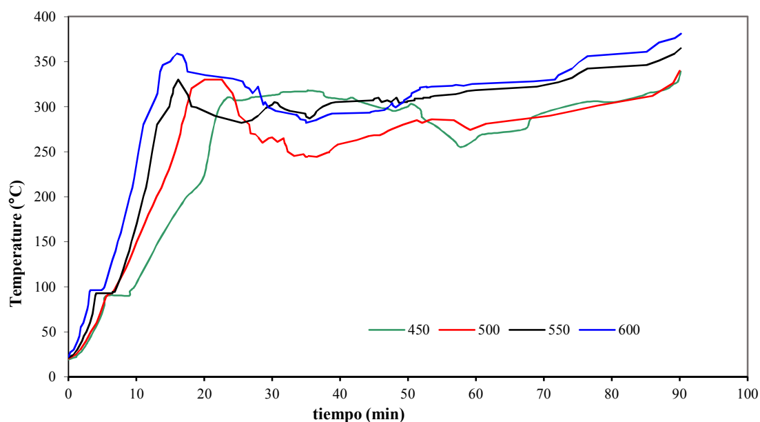
Figure S1. Thermographs measured inside of the reactor at different temperatures without a constant hydrogen flow.
