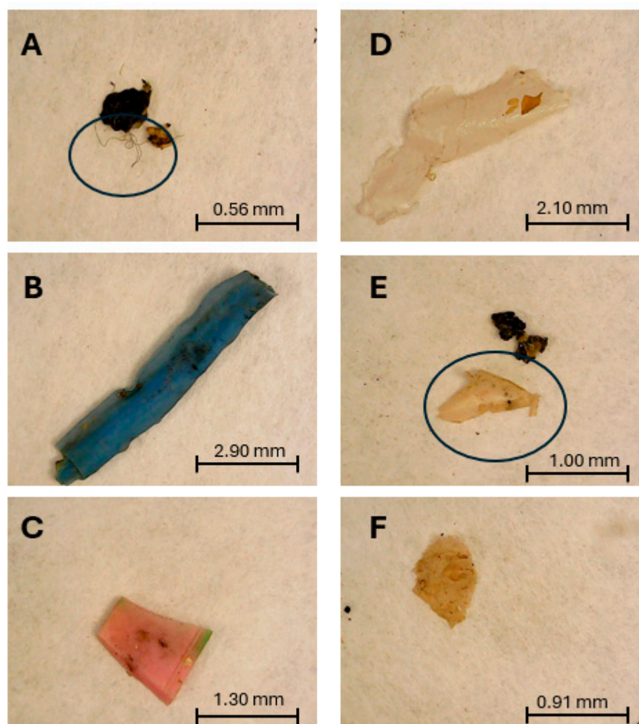
Figure 10. Images of some microplastic fibers (A), fragments (B,C), and films (D–F) recovered from the sediments of the Black Cart and White Cart Waters.
