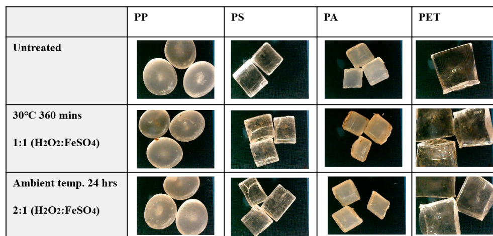
Figure 8. Digital microscope images of microplastics before and after digestion in Fenton's reagent.
