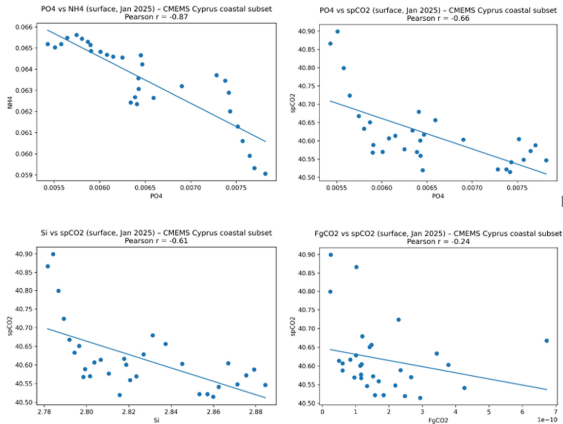
Figure 6. Pairwise correlations between selected biogeochemical parameters in the coastal surface CMEMS proxy dataset for Cyprus (January 2025). Source: CMEMS—Copernicus Marine Environment Monitoring Service, dataset: MEDSEA_ANALYSISFORECAST_BGC_006_014, January 2025, surface layer (surface; ~14 m); Location coordinates: latitude and longitude in the Cyprus coast zone (34.92° N, 33.68° E).
