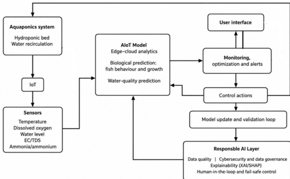
Figure 2. AIoT-based aquaponics monitoring, prediction, and decision-support framework.
