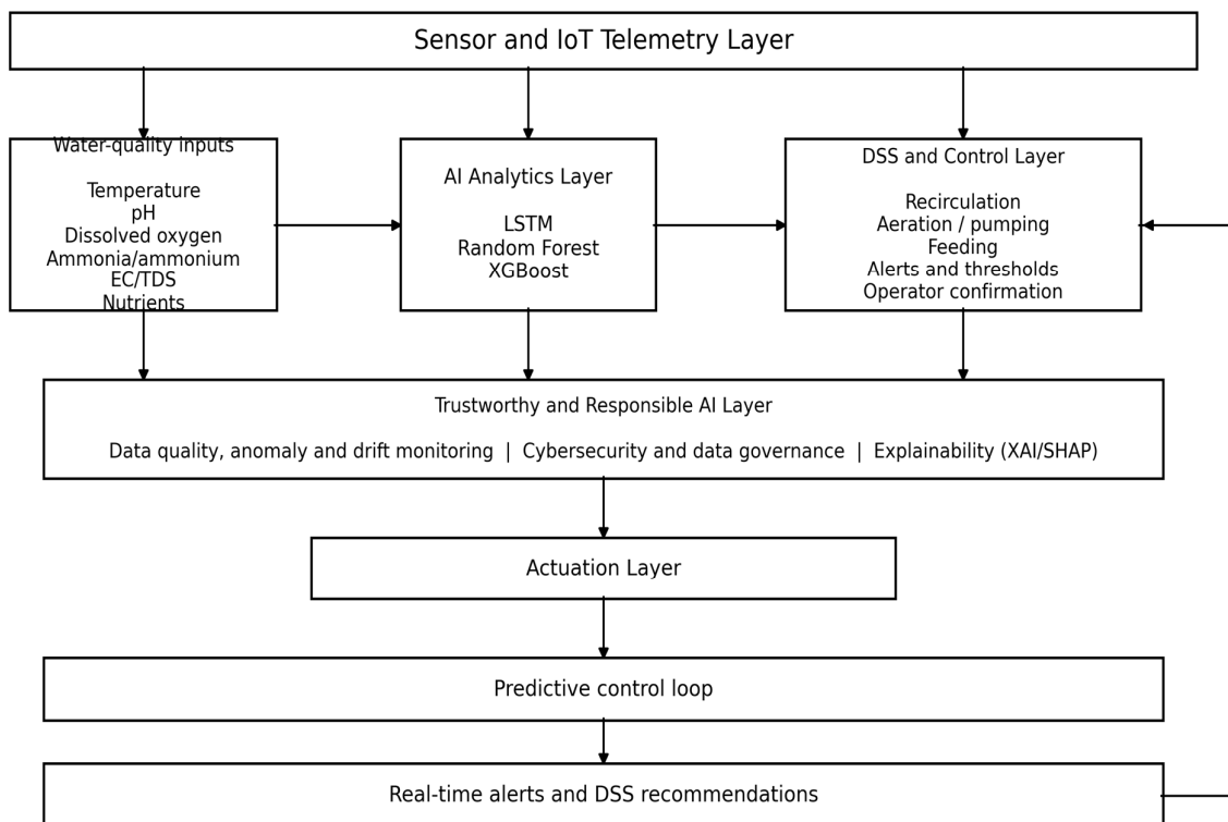
Figure 1. Layered AIoT architecture for aquaponics decision support and responsible control.
