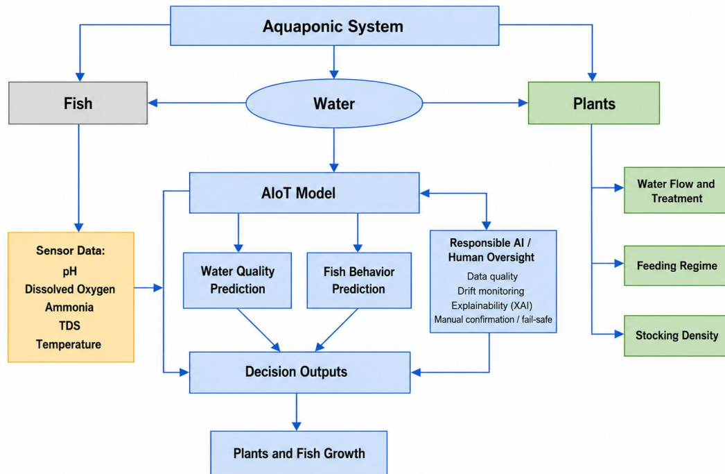
Figure 7. Proposed AIoT model structure for aquaponics monitoring, prediction, and DSS support.
