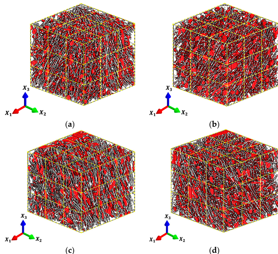
Figure 13. Three-dimensional \mu CT volume view showing internal microstructure (fiber—gray; voids—red) of the various ROI volumes and the RVE-II instances for each: (a) ROI-I, (b) ROI-II, (c) ROI-III and (d) ROI-IV.
