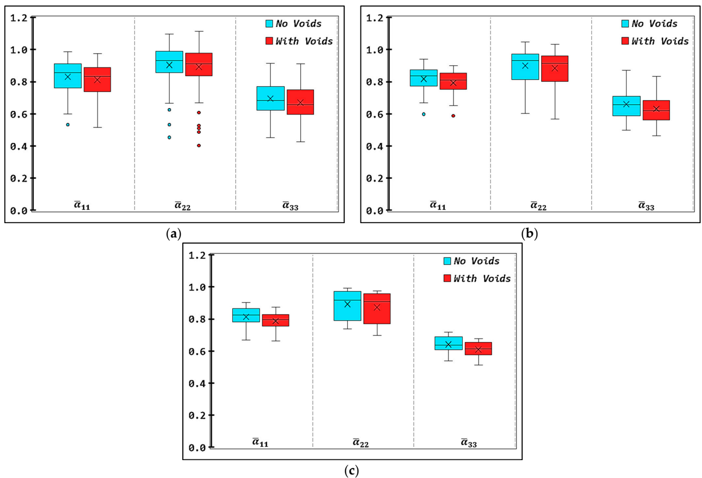
Figure 10. Box plot showing the mean values ('x' markers), median values (horizontal lines), interquartile intervals (box limits), extremums (whiskers) and outliers (isolated points) of the computed components of the normalized effective CTE tensor from the RVE realization datasets for (a) RVE-I, (b) RVE-II and (c) RVE-III. Results are shown for analyzed cases with microvoids (red) and without microvoids (blue) present within the bead's microstructure.
