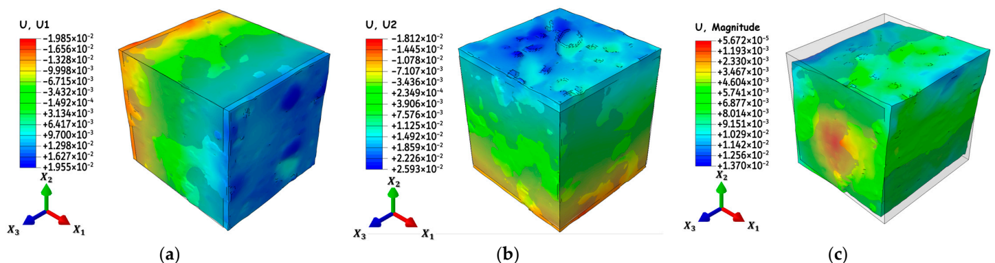
Figure 6. Isometric view of the deformation contours of RVE-II, #14 from ROI-II, overlaid over the undeformed volume under different loading values: (a) tensile response in x_1 -direction; (b) tensile response in x_2 -direction; (c) shear response in x_1x_2 -plane.
