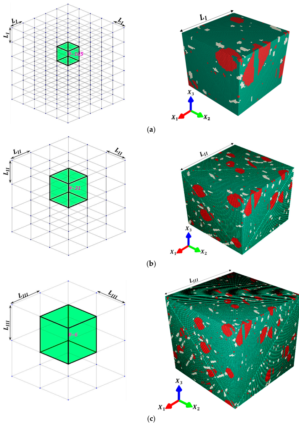
Figure 3. ROI-II partitioning into (a) RVE—I: 125 realizations with 125,000 elements per realization with L_I = 70 \mu\text{m} ; (b) RVE—II: 27 realizations with 571,787 elements per realization with L_{II} = 116.2 \mu\text{m} ; (c) RVE—III: 8 realizations with 1,953,125 elements per realization with L_{III} = 175 \mu\text{m} .
