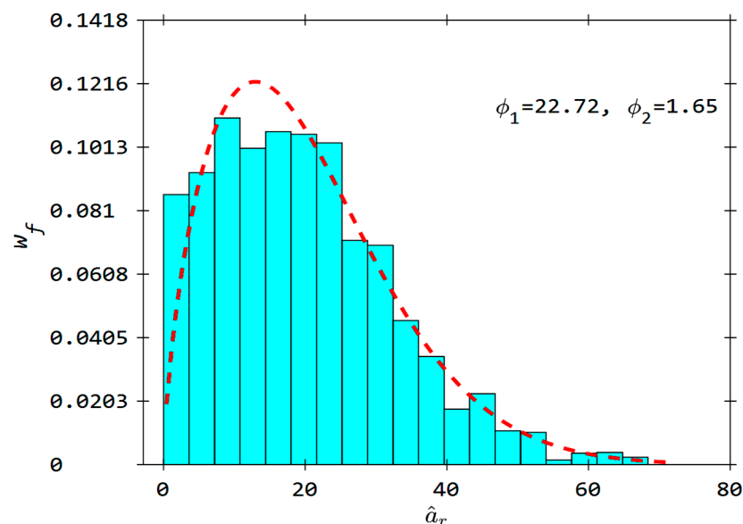
Figure 5. Fiber aspect ratio distribution extracted for ROI-II. (red dashed line represents the fitted Weibull distribution function curve)
