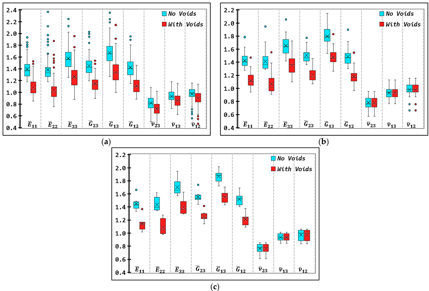
Figure 8. Box plot showing the mean values ('x' markers), median values (horizontal lines), interquartile intervals (box limits), extremums (whiskers) and outliers (isolated points) of the computed normalized engineering constants from RVE realization datasets for (a) RVE-I, (b) RVE-II and (c) RVE-III. Results are shown for analysis cases with micro-voids (red) and without micro-voids (blue) present within the bead's microstructure.
