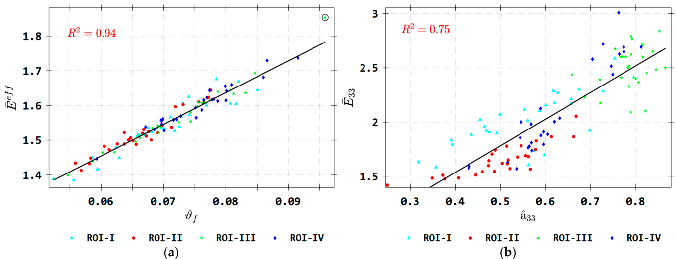
Figure 14. Linear correlation plots between (a) the effective elastic modulus \bar{E}^{eff} and the fiber volume fraction \vartheta_f and between (b) the elastic modulus component \bar{E}_{33} and the average fiber orientation tensor component \hat{a}_{33} for non-porous RVE-II instances of the various ROIs. (circled markers indicate outlier datapoints).
