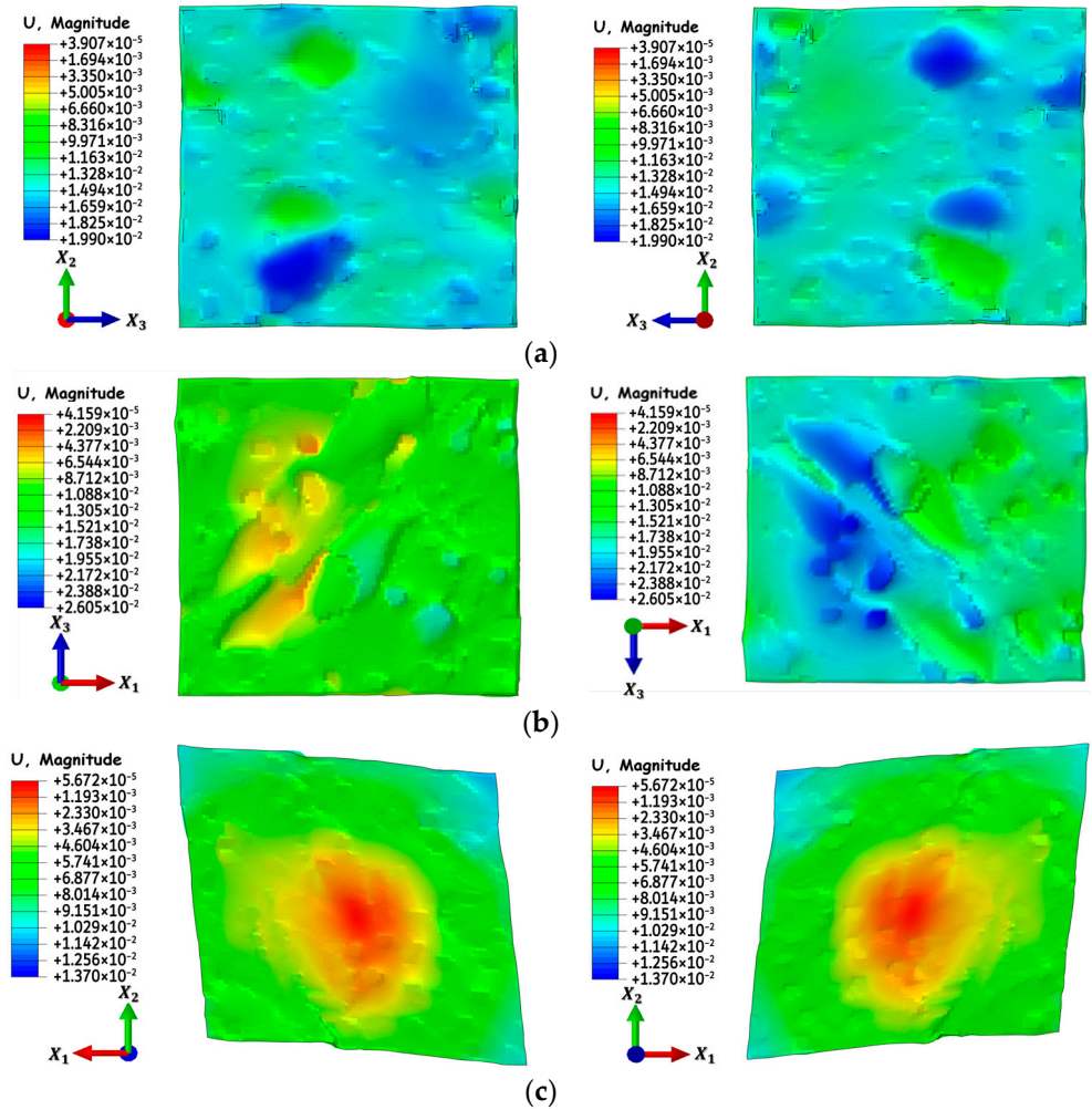
Figure 7. Deformation contours of RVE-II, #14 from ROI-II, showing the topography of opposing bounding face pairs to validate the implementation of PBC for loading in the (a) x_1 -direction, (b) x_2 -direction and (c) x_1x_2 -plane. The images show RVE bounding faces in the negative (left column) and positive (right column) direction (or normal in case of shear) to the direction of the applied loading.
