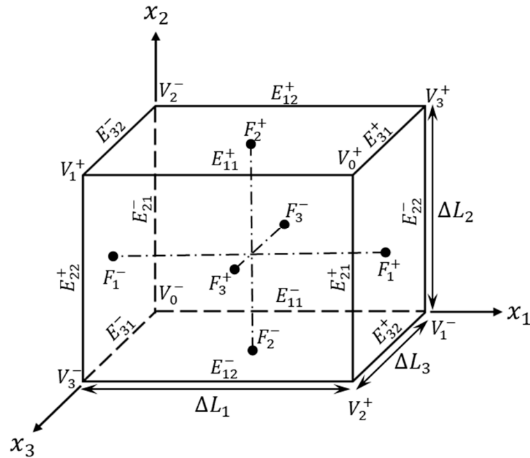
Figure 4. Single periodic RVE structure showing definitions of entities and coordinate directions used in the PBC formulations (Equations (1)–(3)).
