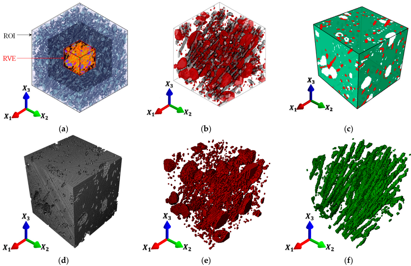
Figure 2. (a) Reconstructed \mu CT 3D scans of ROI-II highlighting mid-block RVE volume; (b) magnified view of mid-block RVE showing segmented micro-constituents; (c) FEA model imported from \mu CT voxel data of the RVE; (d) ABS matrix FEA elements; (e) micro-void FEA elements; and (f) fiber reinforcement FEA elements.
