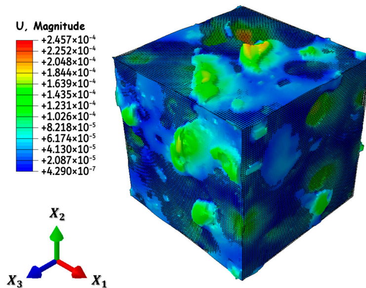
Figure 9. Deformation contour of RVE-II, #14 from ROI-II region, overlaid on the undeformed mesh geometry and showing the bulk response of the volume under thermal load of \Delta\theta = 65^\circ\text{C} .
