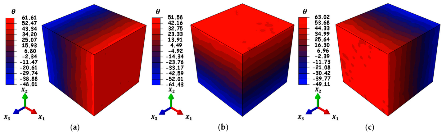
Figure 11. Temperature contours of RVE-II, realization #14 from ROI-II, for three thermal load conditions: (a) thermal gradient in x_1 -direction, (b) thermal gradient in x_2 -direction and (c) thermal gradient in x_3 -direction. Units of \theta in ^{\circ}\text{C} .
