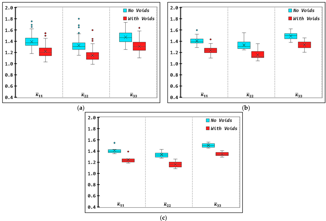
Figure 12. Box plot showing the mean values ('x' markers), median values (horizontal lines), inter-quartile intervals (box limits), extremums (whiskers) and outliers (isolated points) of the diagonal components of the normalized effective TC tensor from the RVE realizations for (a) RVE-I, (b) RVE-II and (c) RVE-III. Results are shown for the analyzed cases with micro-voids (red) and without micro-voids (blue) present within the bead's microstructure.
