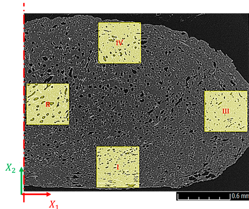
Figure 1. Regions of interest (ROI, I–IV) of the CF/ABS specimen from a polymer composite bead manufactured using Baylor’s LAAM system. ( X_1 and X_2 are coordinate directions normal to the print direction, X_3 , and the red dot dashed line indicates a plane of half-symmetry plane in the X_1 direction.)
