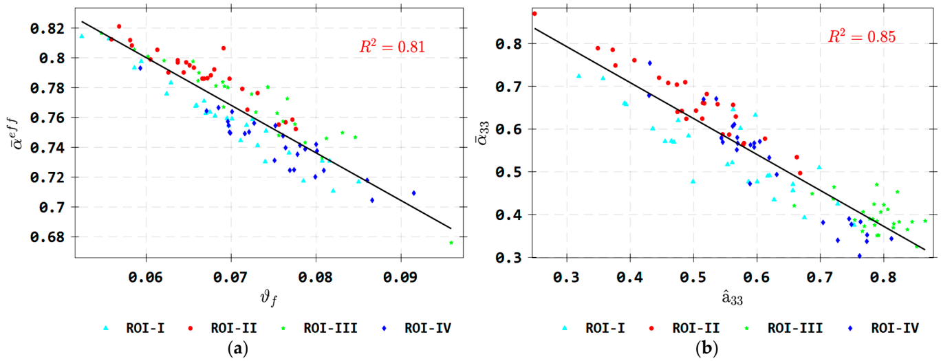
Figure 15. Linear correlation plots between (a) the apparent ECTE magnitude \bar{\alpha}^{eff} with the fiber volume fraction \vartheta_f and between (b) the ECTE tensor component \bar{\alpha}_{33} and the average fiber orientation tensor component \hat{a}_{33} for non-porous RVE-II instances of the various ROIs.
