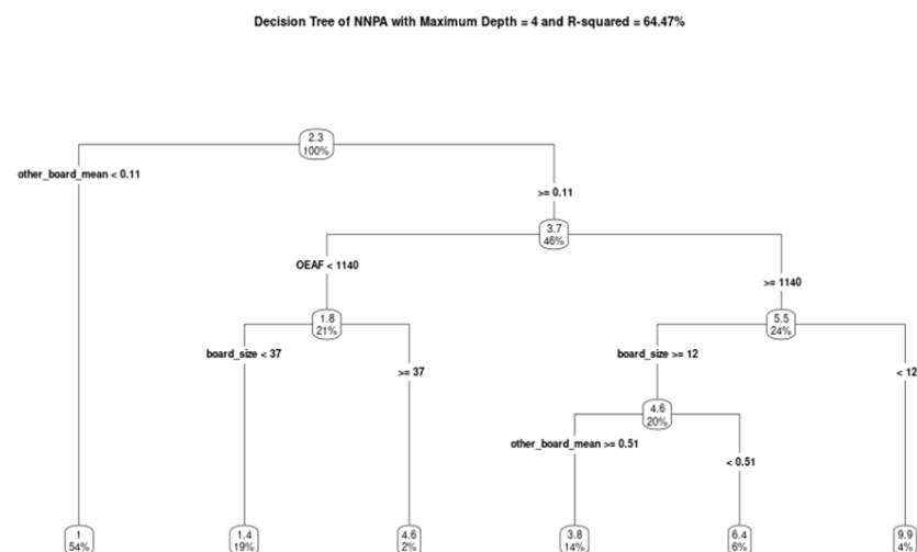
Figure 3. Decision tree of solvency risk. General notes: Figure 3 illustrates the decision tree branches using 4 levels of branches (maximum depth = 4) to display how the average value of the dependent variable, Solvency Risk = net non-performing assets, NNPA (log value of net non-performing assets in millions of Indian Rupees), is influenced by different threshold values of independent variables associated with 37 Indian commercial banks between 2006 and 2018. Variable definitions: other_board_mean = Average number of other board memberships held by directors (director "Busyness" indicator); OEAF = Auditors' fees and expenses (in millions of Indian rupees, INR); and board_size = number of board members.
