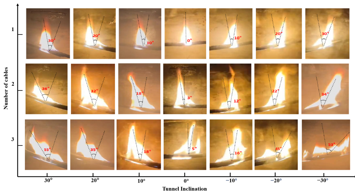
Figure 8. Flame morphology variation in cable combustion under windless conditions.
