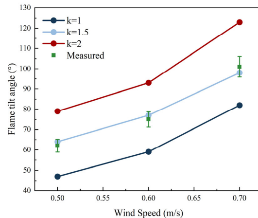
Figure 10. Sensitivity analysis of empirical coefficient k .
