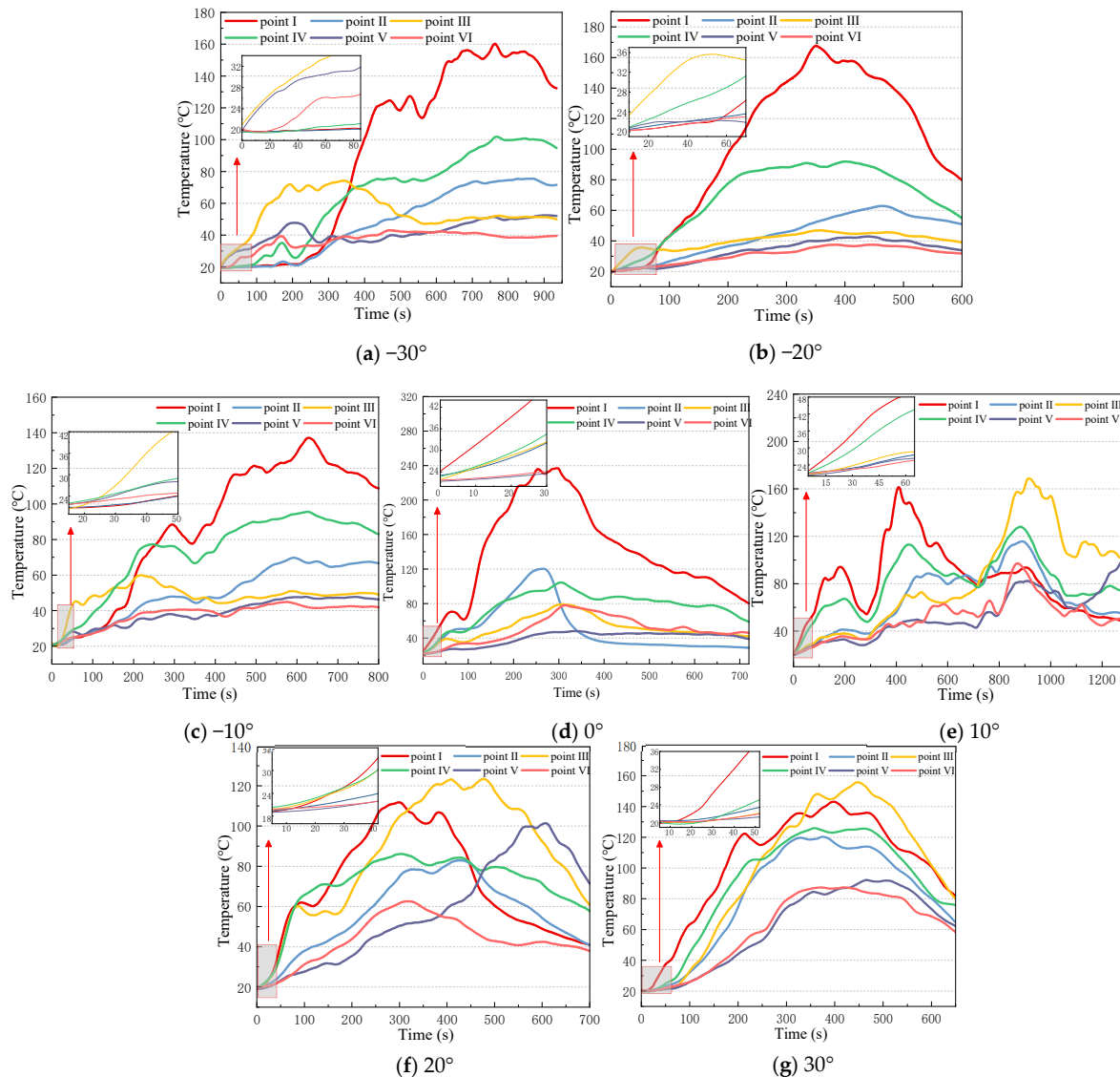
Figure 15. Temperature variation near the fire source in cable combustion under windless conditions.
