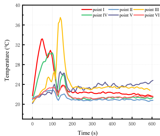
Figure 17. Temperature variation near the fire source under 0.5 m/s wind speed and 0^\circ tilt angle.
