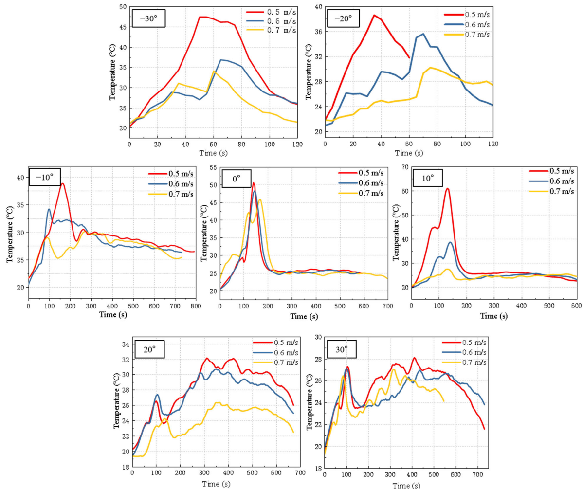
Figure 18. Temperature variation near the fire source during cable combustion under windy conditions.
