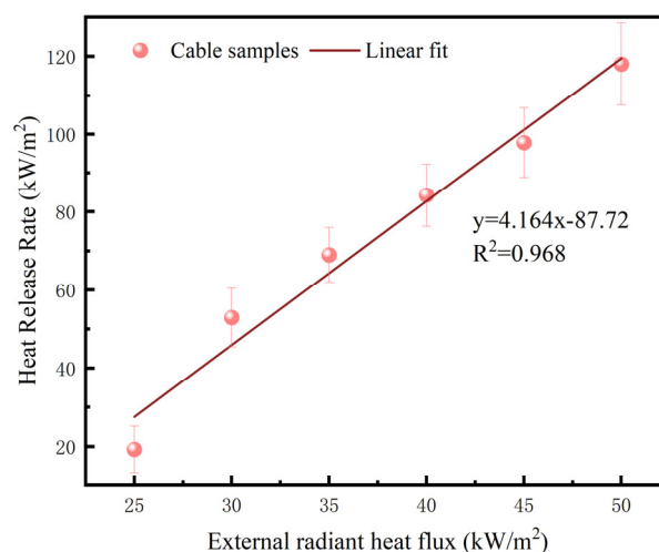
Figure 7. Correlation between external radiant heat flux and maximum HRR peak of the cable.
