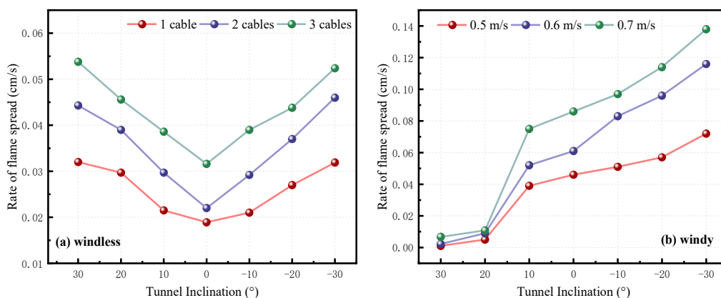
Figure 14. Flame spread rates of cable combustion under windless and ambient wind conditions.
