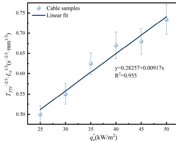
Figure 5. Linear fitting of T_{TII}^{-2/3} \cdot L_0^{1/3} and q_e'' .
