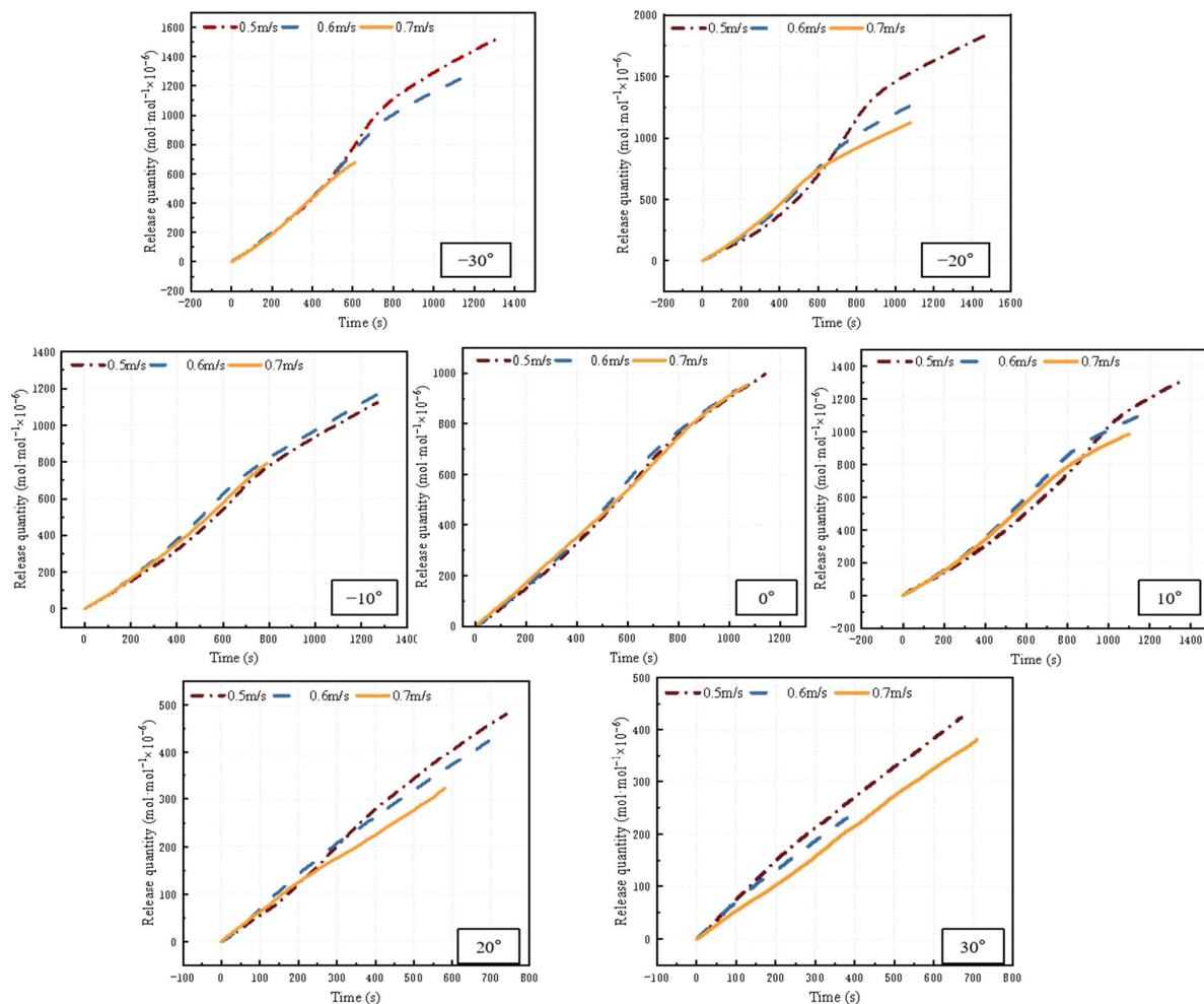
Figure 19. CO gas release under varying ambient wind speeds.
