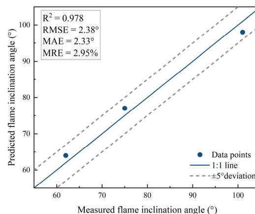
Figure 11. Comparison between measured and predicted flame inclination angles.
