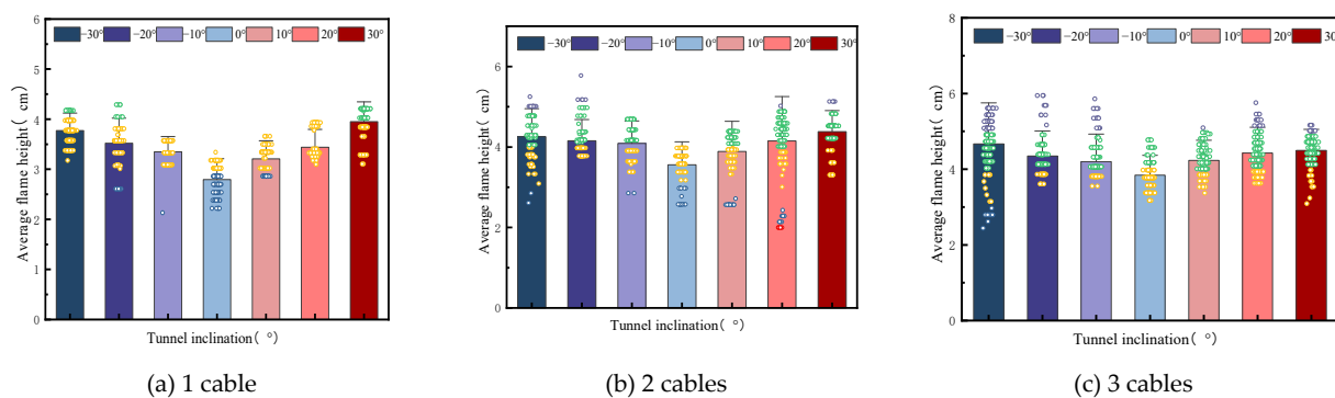
Figure 12. Average flame height in cable combustion under windless conditions.
