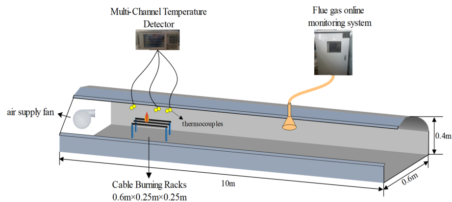
Figure 1. Simplified diagram of the experimental platform.
