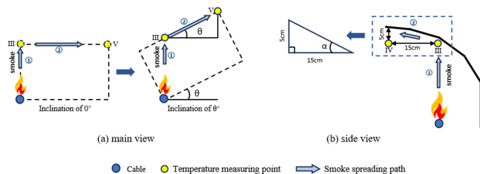
Figure 16. Schematic diagram of smoke spread under negative tilt angles.
