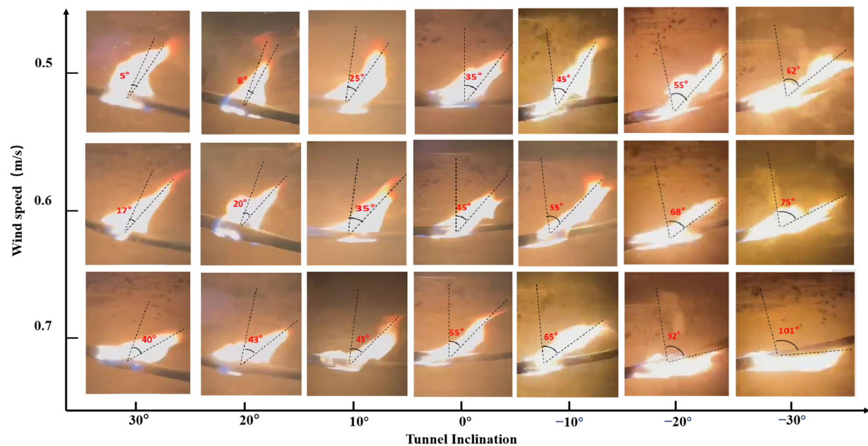
Figure 9. Flame morphology variation in Cable Combustion under windy conditions.
