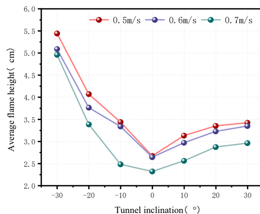
Figure 13. Average flame height in cable combustion under windy conditions.
