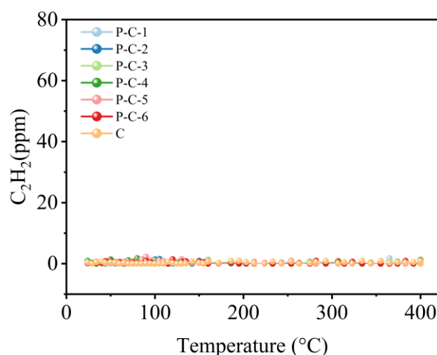
Figure 7. C_2H_2 gas release pattern during spontaneous combustion of mixed samples.
