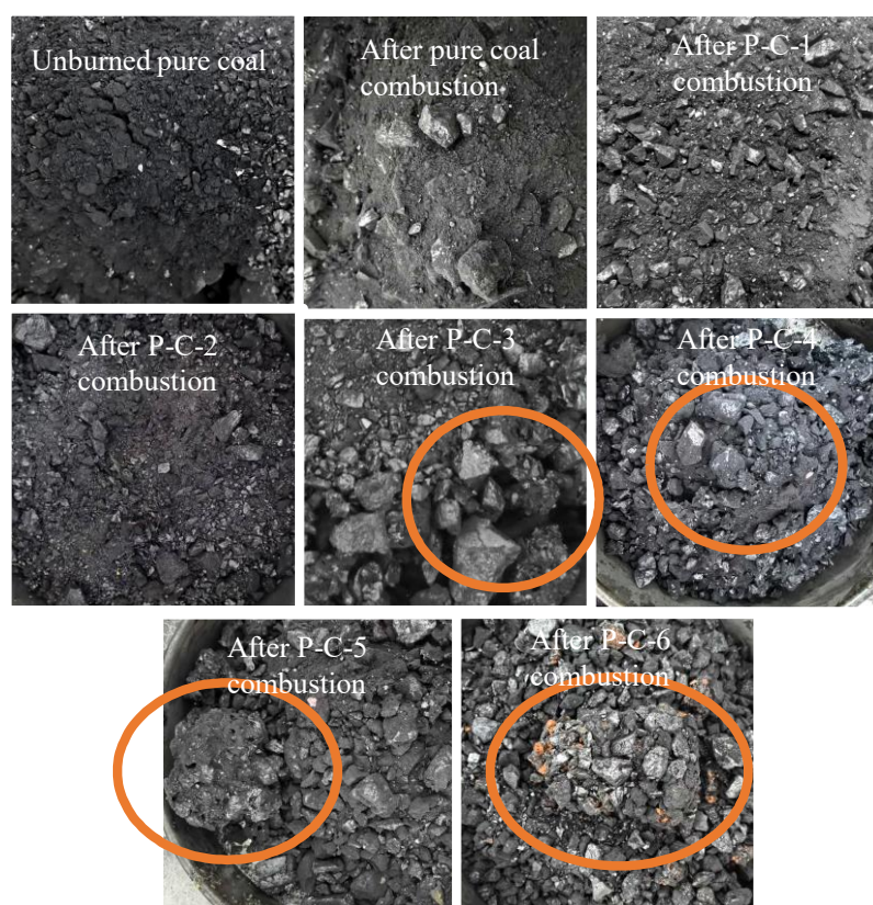
Figure 9. Surface morphology of the pure coal sample before and after combustion and of mixed samples after combustion.
