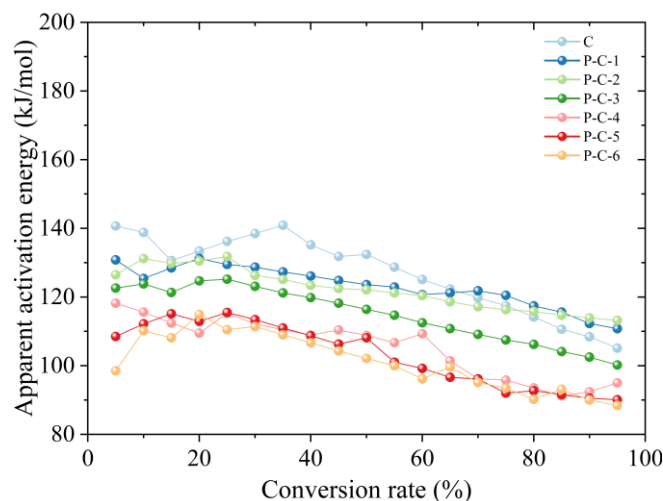
Figure 11. Variation trend of apparent activation energy of coal-PU mixed samples based on the DAEM model.
