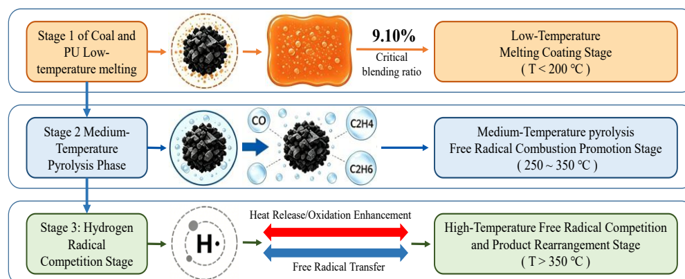
Figure 12. Schematic diagram illustrating the mechanism of the coal-PU synergistic self-ignition effect.
