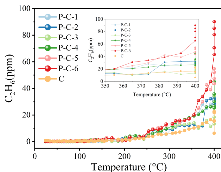
Figure 6. C_2H_6 gas release pattern during spontaneous combustion of mixed samples.
