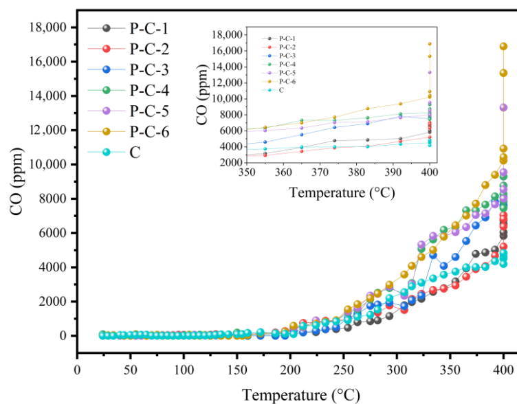
Figure 3. CO gas release pattern during spontaneous combustion of mixed samples.
