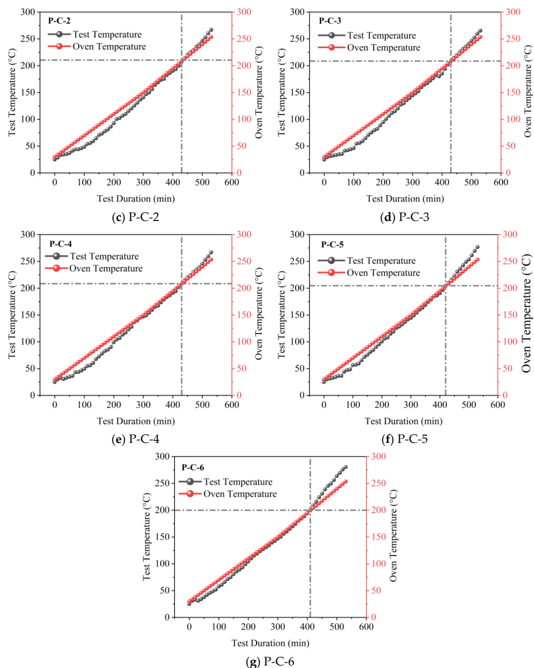
Figure 8. Temperature trends during spontaneous combustion of coal and mixed samples.
