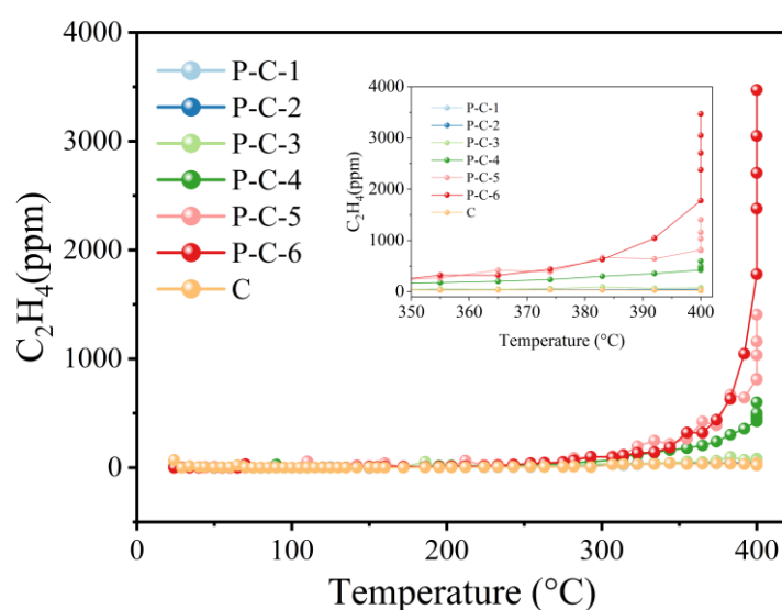
Figure 5. C_2H_4 gas release pattern during spontaneous combustion of mixed samples.
