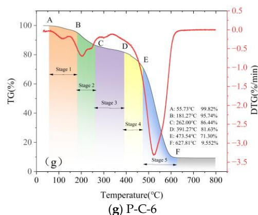
Figure 10. TG-DTG curves of mixed samples with different proportions at a heating rate of 5 K/min.
