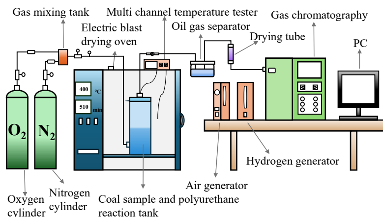
Figure 1. Schematic diagram of the programmed heating and gas chromatography experimental system.
