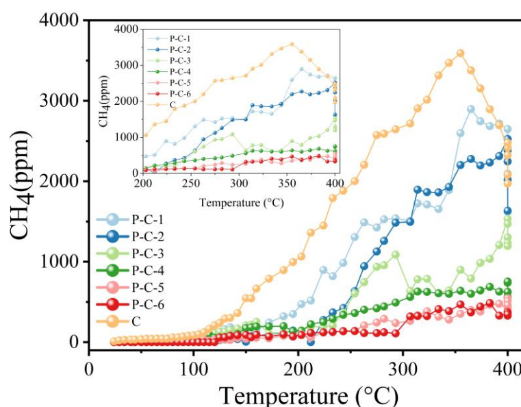
Figure 4. CH 4 gas release pattern during spontaneous combustion of mixed samples.
