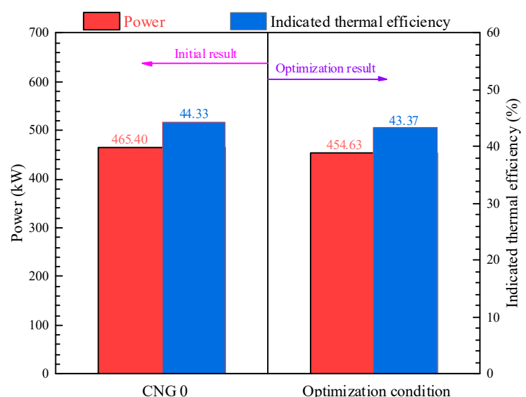
(a) Comparison of power and ITE
