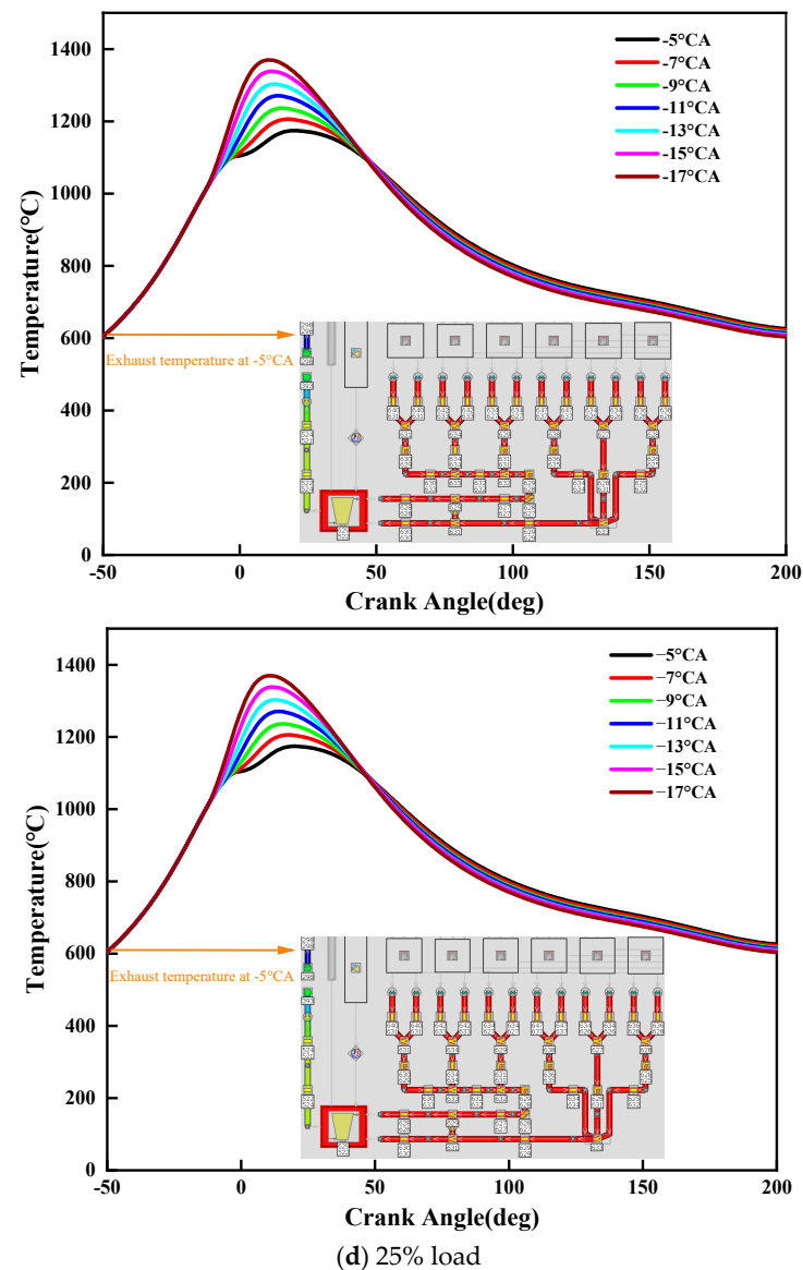
Figure 13. Effect of diesel injection timing on in-cylinder temperature at (a) 100%, (b) 75%, (c) 50%, and (d) 25% engine load.
