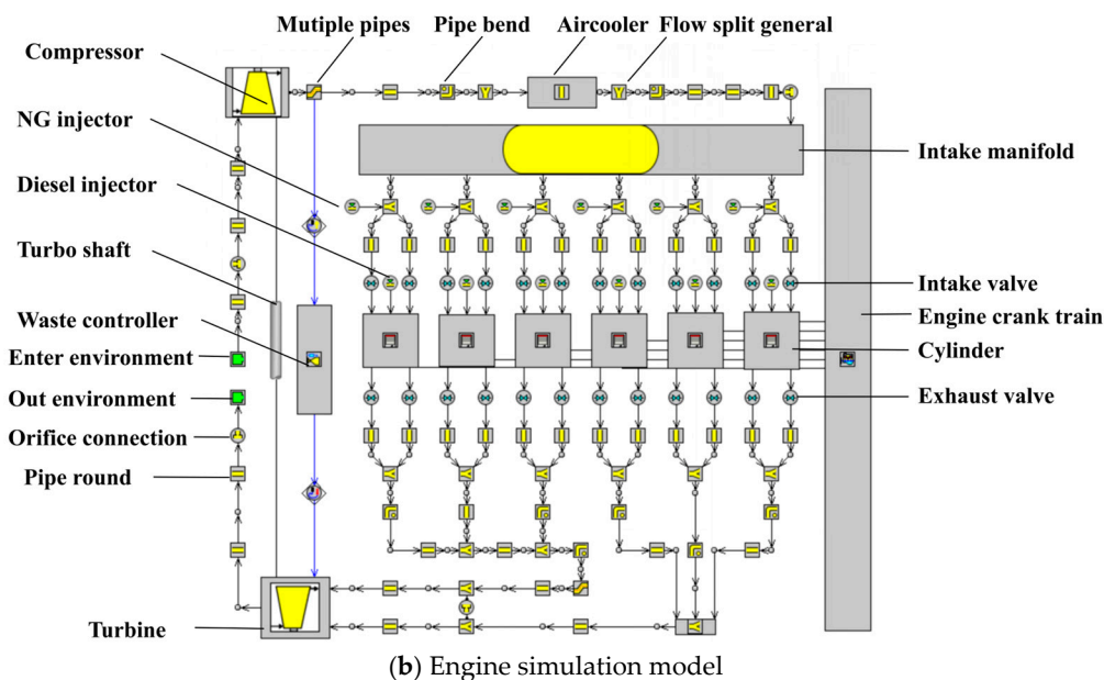
Figure 1. Engine physical model and simulation model.
