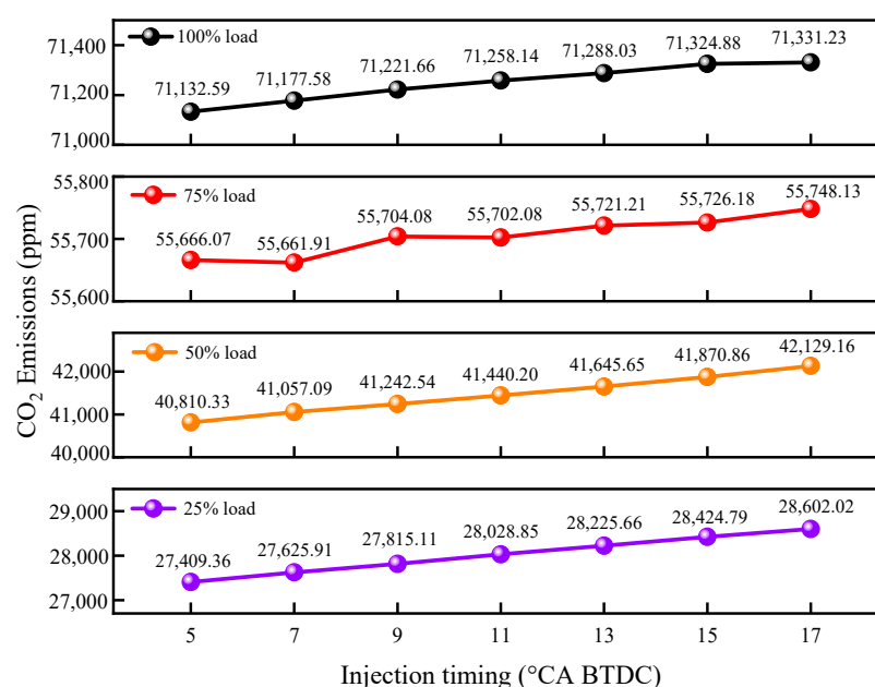
Figure 18. Effect of diesel injection timing on \text{CO}_2 emissions under four engine load conditions.
