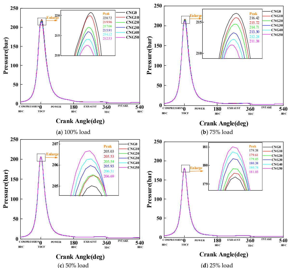
Figure 4. Effect of natural gas substitution rate on in-cylinder pressure at (a) 100%, (b) 75%, (c) 50%, and (d) 25% engine load.
