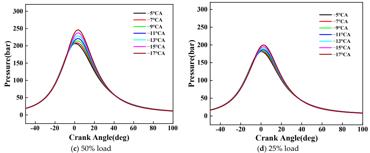
Figure 12. Effect of diesel injection timing on in-cylinder pressure at (a) 100%, (b) 75%, (c) 50%, and (d) 25% engine load.
