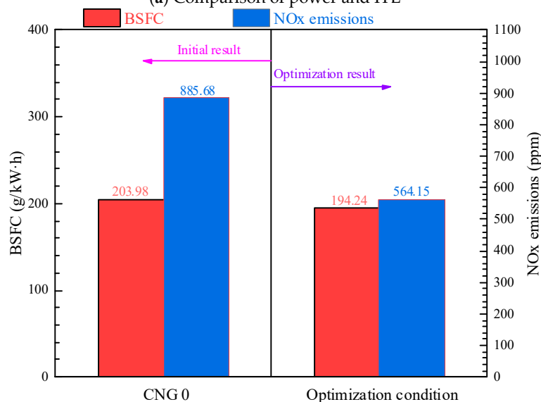
(b) Comparison of BSFC and NO x emissions
