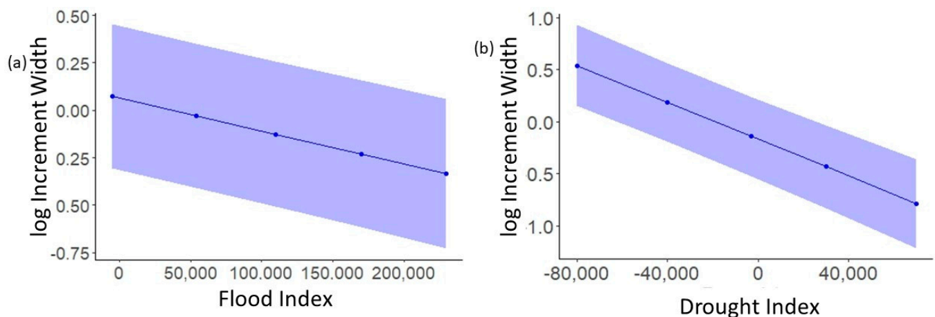
Figure 7. Mixed-effects models of flood (a) and droughts indices (b) in relation to log (increment width) for P. fasciatus in the Amazon basin. Higher F and D indices corresponded to a decrease in the increment width.
