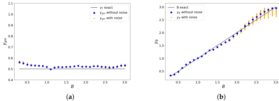
Figure 14. Estimated ( y_{gm} , y_B ) versus exact values of the Greitzer parameter B and throttle setting \gamma_T for the 10% dataset, including sensor accuracy of 10% of the measured value, simulated by noise addition.
