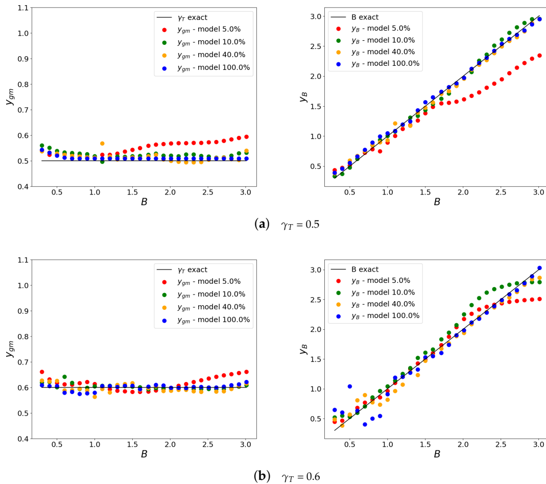
Figure 8. Estimated (y_{gm}, y_B) versus exact values of the Greitzer parameter B and throttle setting \gamma_T for input time sequences of different lengths.
