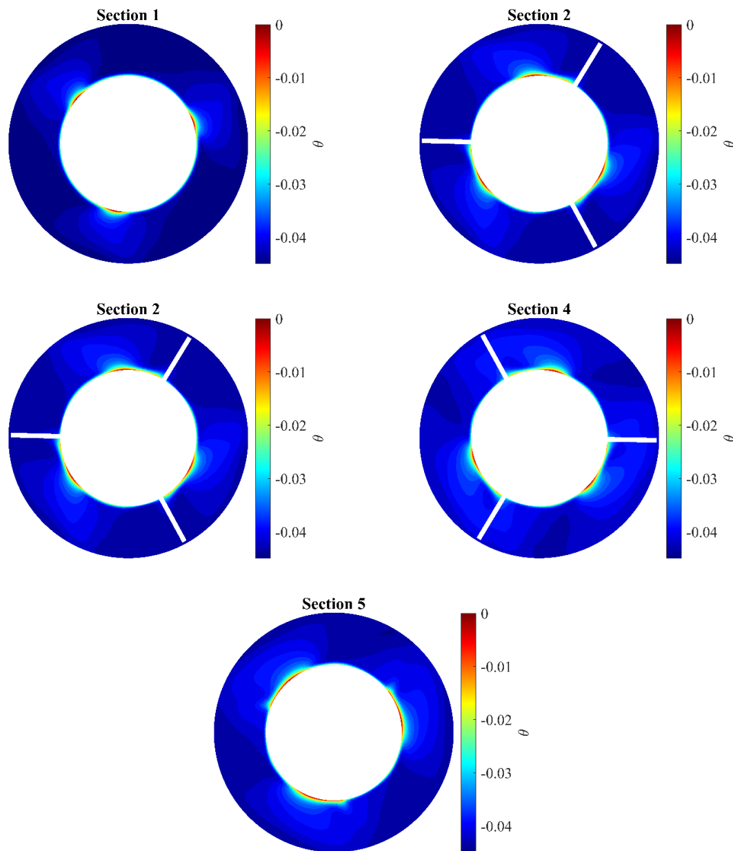
Figure 10. Fluid dimensionless temperature distributions (sections of Figure 6).
