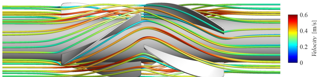
Figure 7. Streamlines at Re_g = 4.9 .
