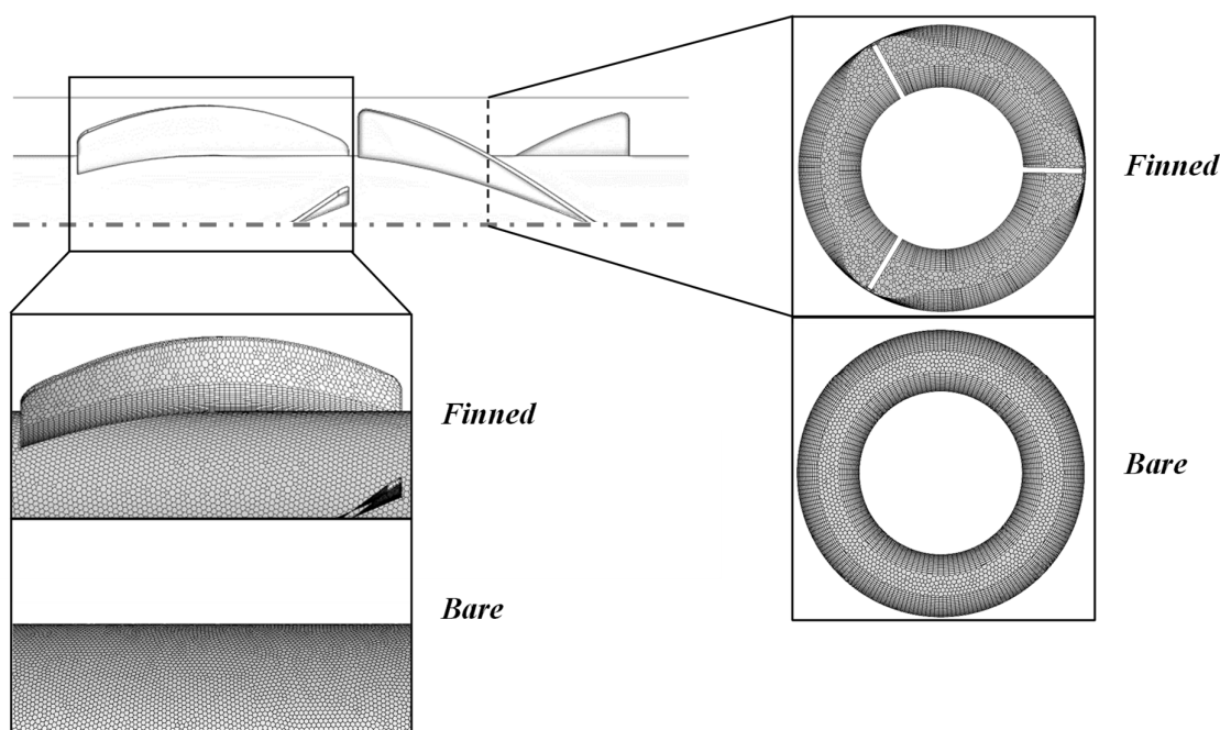
Figure 3. Details on the adopted meshing strategy for the finned and bare annuli.
