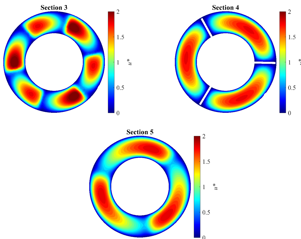
Figure 9. Dimensionless fluid velocity (sections of Figure 6).
