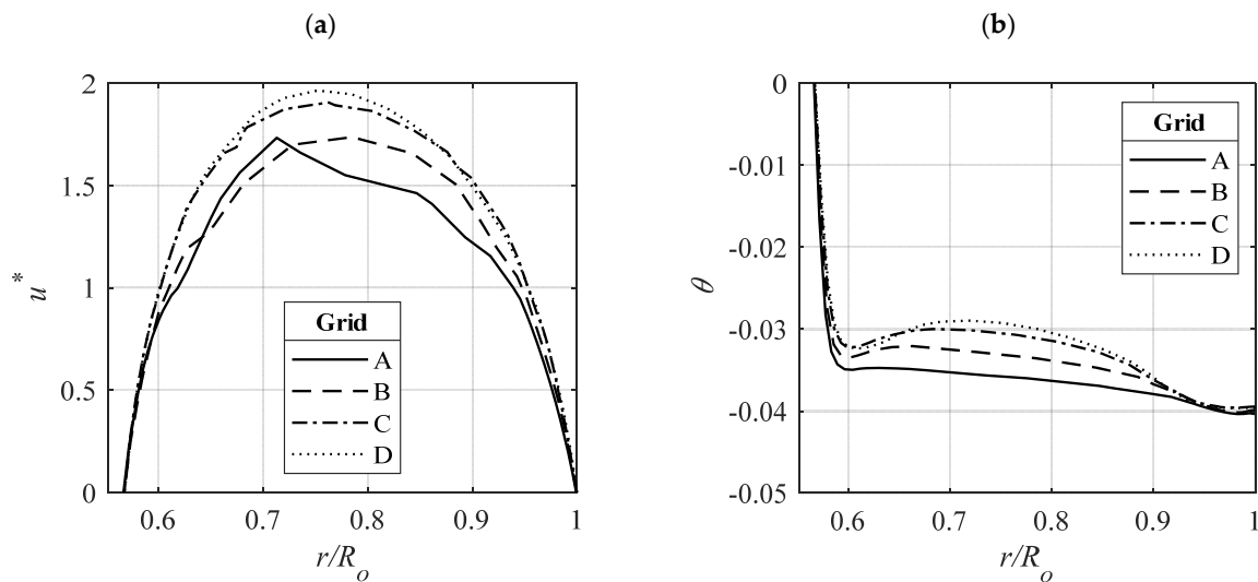
Figure 5. Grid independence analysis for the finned annulus in terms of the dimensionless velocity (a) and dimensionless temperature (b) profiles.
