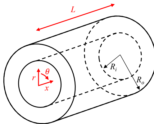
Figure 2. Annular pipe and reference system.
