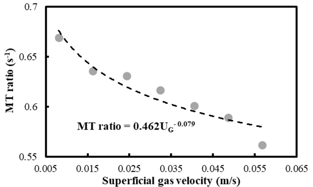
Figure 5. Profile of the MT ratio as a function of U_G in the air–ethylacetate system.
