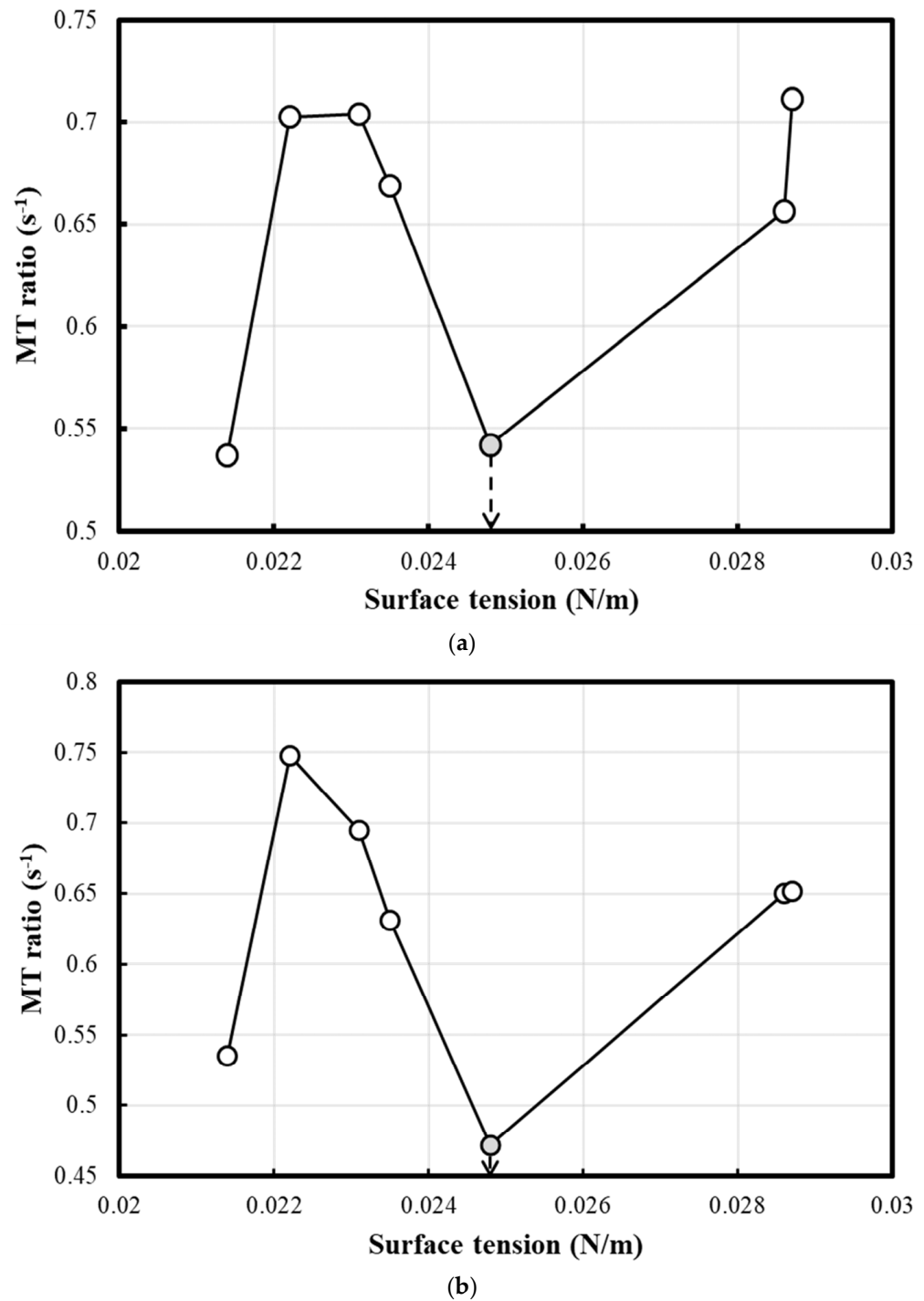
Figure 15. (a) Profile of the MT ratio as a function of the surface tension at U_G = 0.0082 m/s. (b) Profile of the MT ratio as a function of the surface tension at U_G = 0.0162 m/s.
