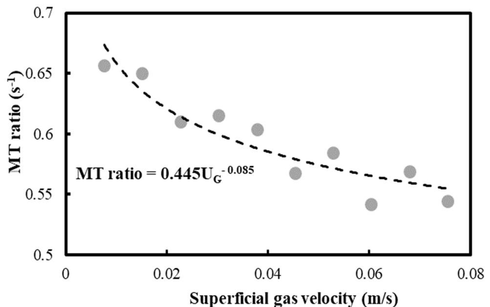
Figure 6. Profile of the MT ratio as a function of U_G in the air–ethylbenzene system.
