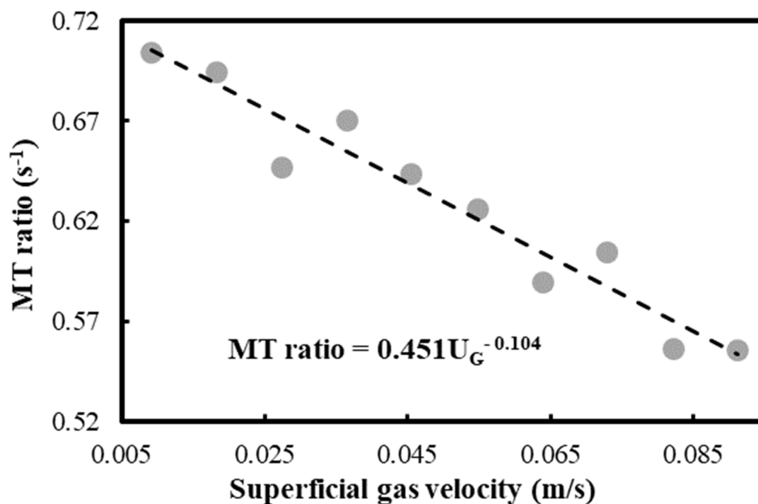
Figure 1. Profile of the MT ratio as a function of U_G in the air–acetone system.
