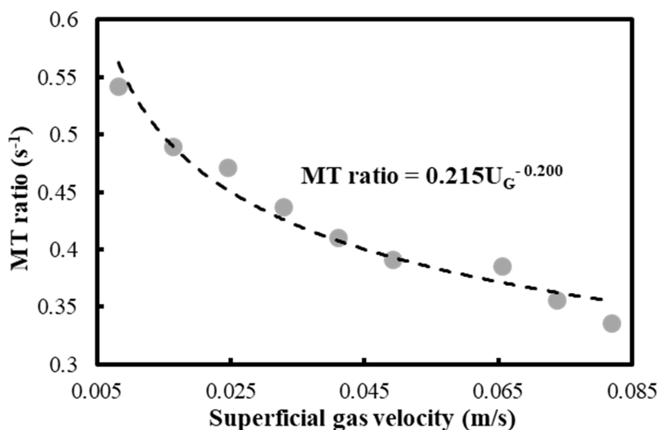
Figure 4. Profile of the MT ratio as a function of U_G in the air–cyclohexane system.
