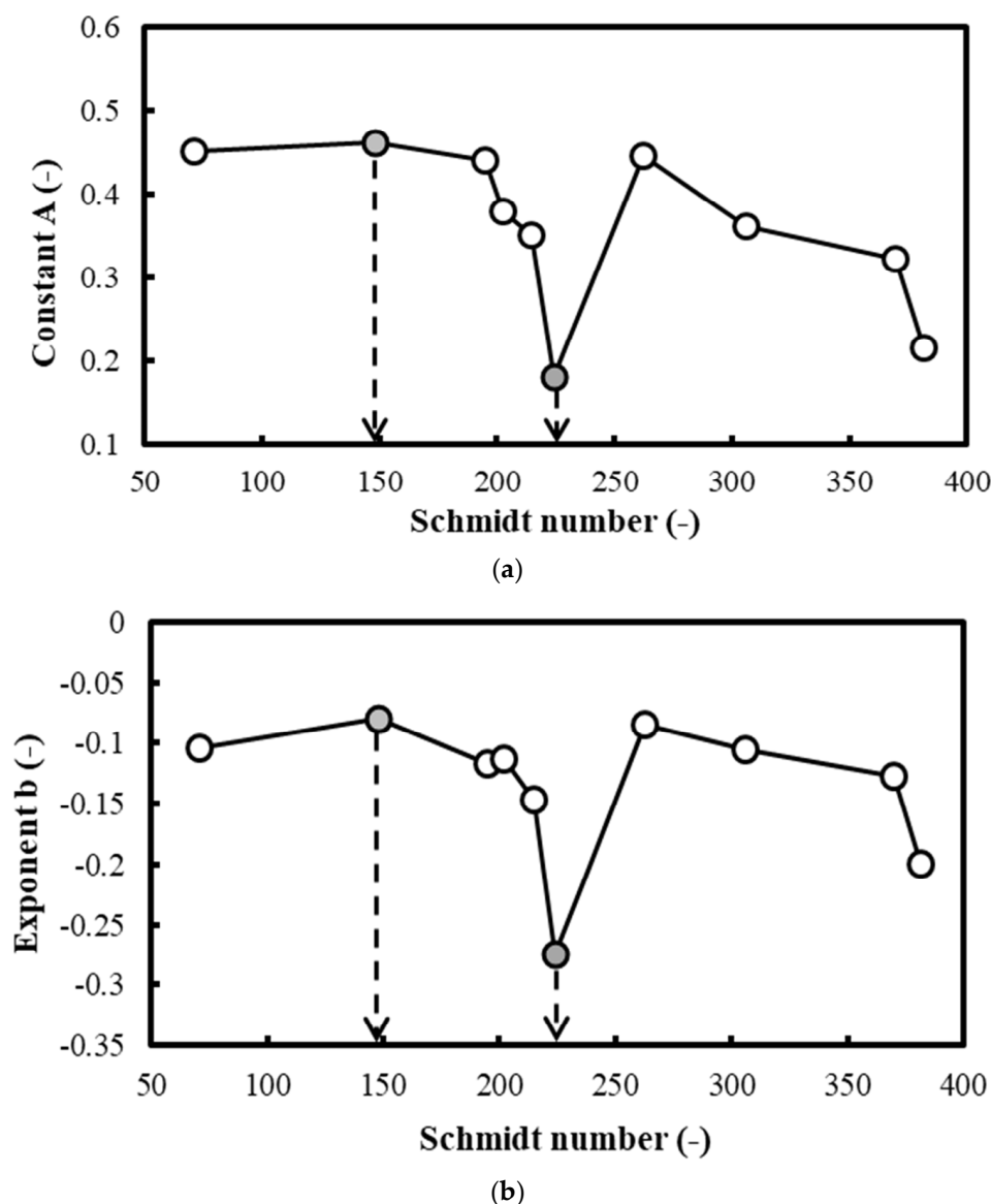
Figure 13. (a) Profile of the constant A as a function of the Schmidt number Sc . (b) Profile of the exponent b as a function of the Schmidt number Sc .
