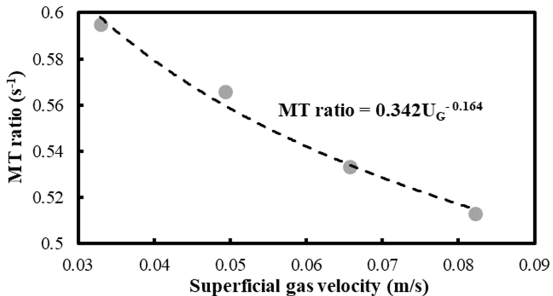
Figure 9. Profile of the MT ratio as a function of U_G in the 6.7% benzene–cyclohexane mixture.
