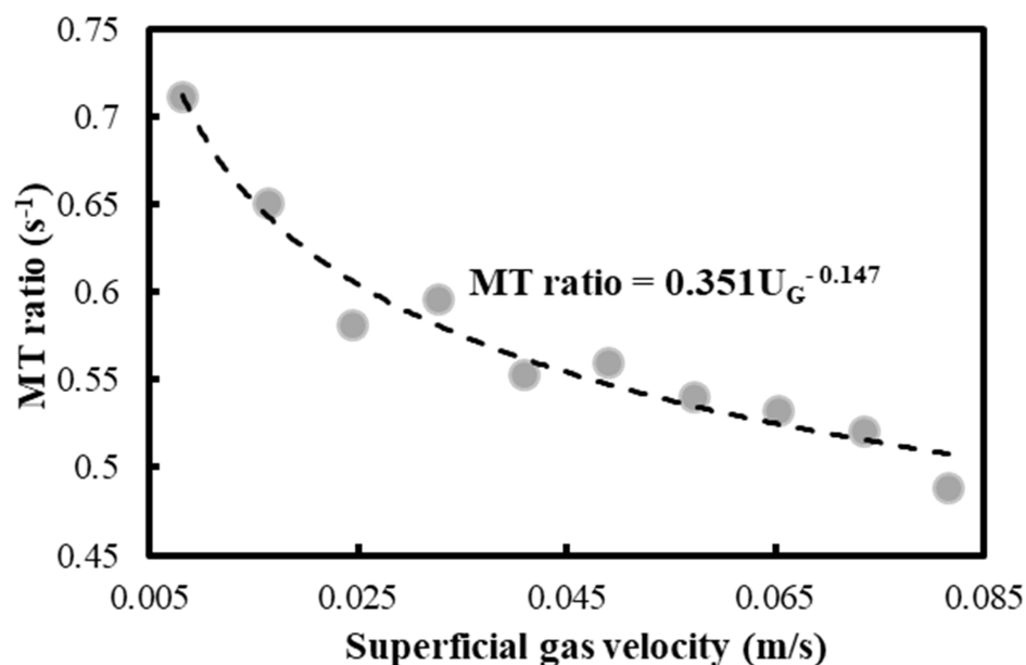
Figure 3. Profile of the MT ratio as a function of U_G in the air–benzene system.
