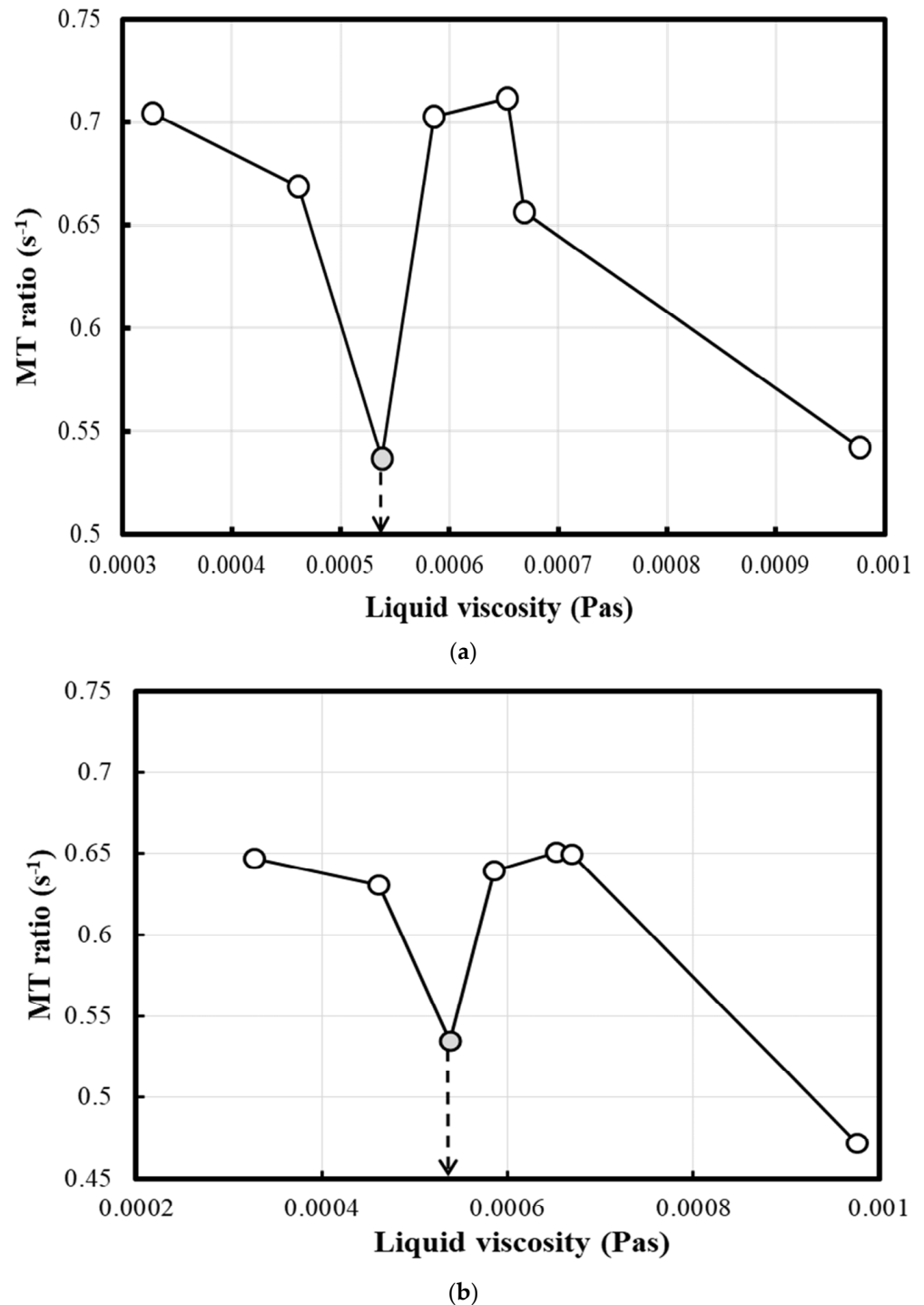
Figure 14. (a) Profile of the MT ratio as a function of the liquid viscosity at U_G = 0.0082 m/s. (b) Profile of the MT ratio as a function of the liquid viscosity at U_G = 0.0163 m/s.
