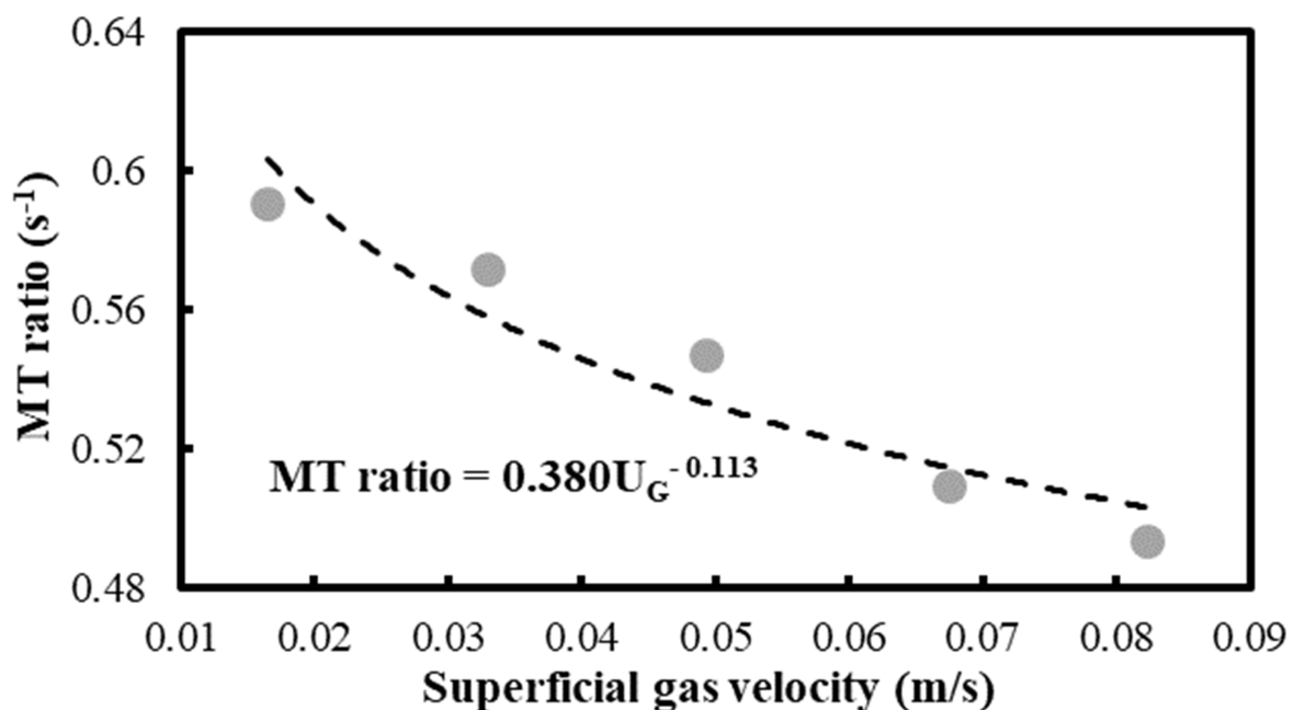
Figure 10. Profile of the MT ratio as a function of U_G in the 13.4% benzene–cyclohexane mixture.
