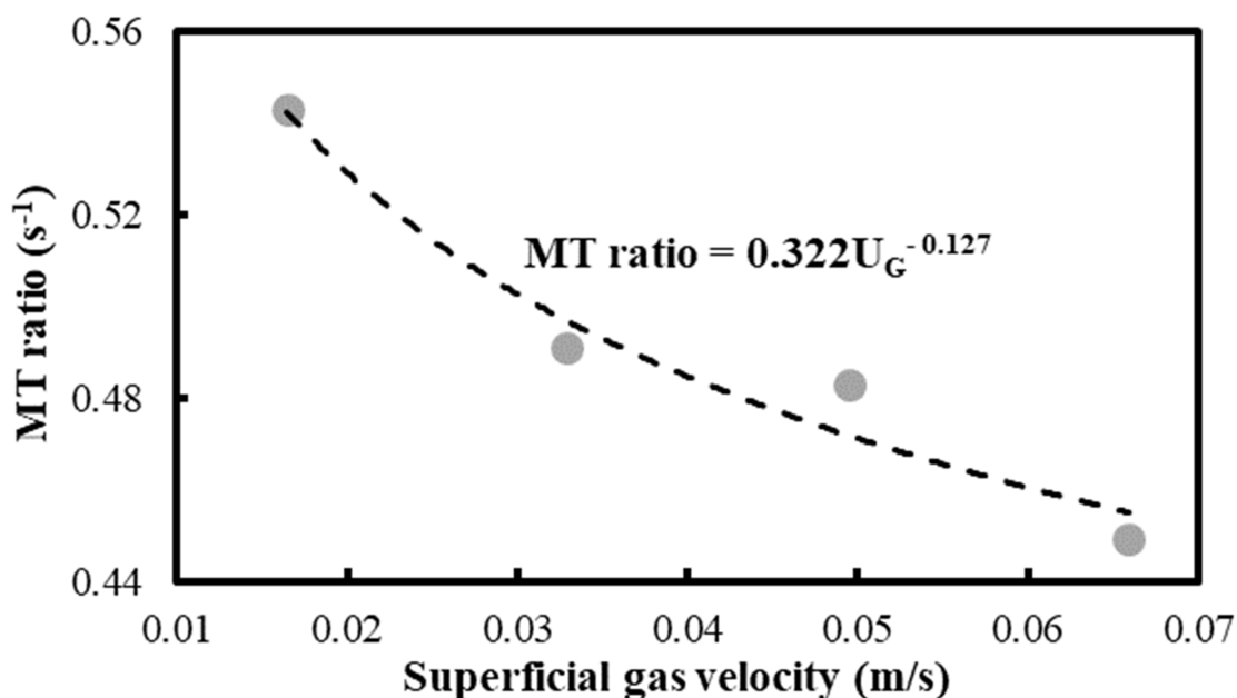
Figure 12. Profile of the MT ratio as a function of U_G in the 90.0% benzene–cyclohexane mixture.
