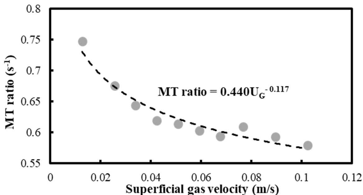
Figure 7. Profile of the MT ratio as a function of U_G in the air–methanol system.
