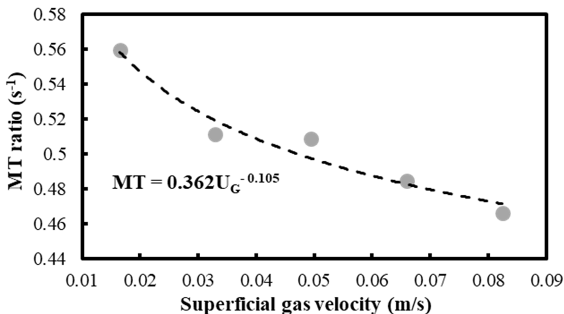
Figure 11. Profile of the MT ratio as a function of U_G in the 78.5% benzene–cyclohexane mixture.
