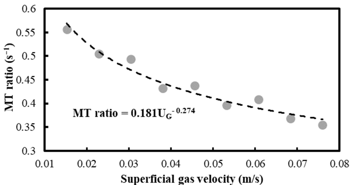
Figure 8. Profile of the MT ratio as a function of U_G in the air–ligroin system.
