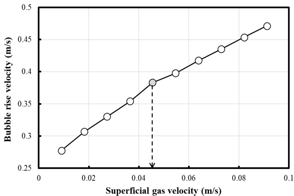
Figure 2. Profile of the MT ratio as a function of U_G in the air–acetone system. Variation of the bubble rise velocity as a function of superficial gas velocity U_G in the air–acetone system.
