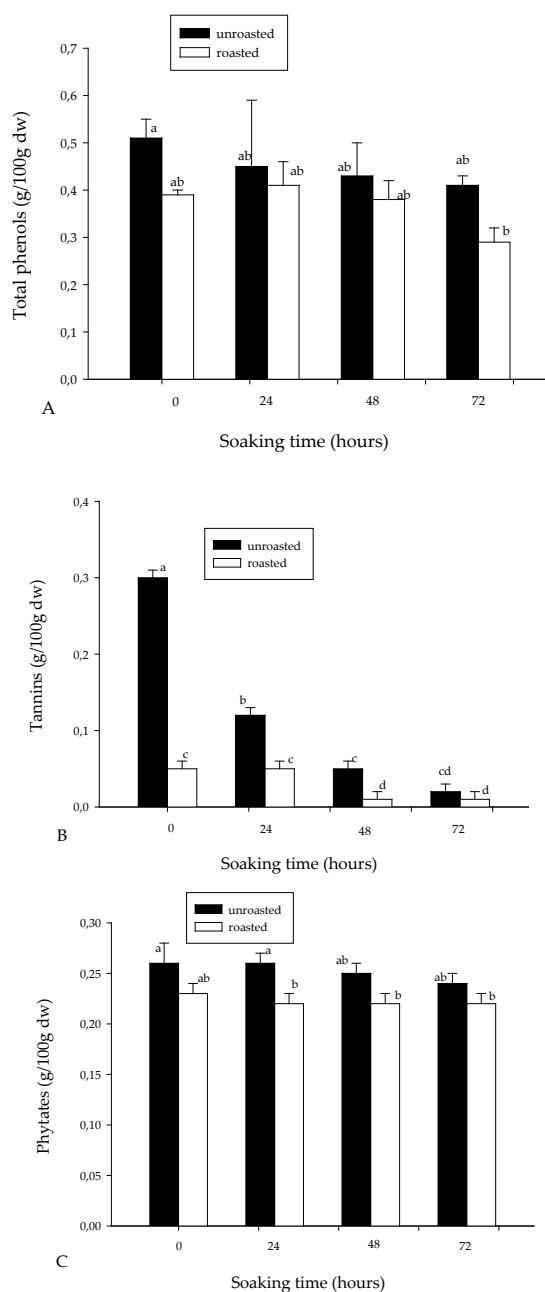
Figure 2. Total (A) polyphenol; (B) tannin; and (C) phytate contents of soybean flour as affected by soaking time and roasting. Bars bearing different letters are significantly different at p < 0.05 ; n = 3 . DW: dry weight.
