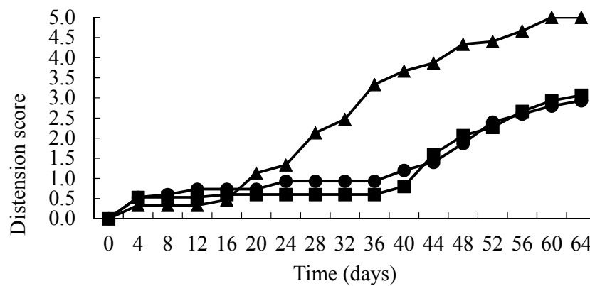
Figure 1. Distension status over time (days) of vacuum packs inoculated with spores of C. estertheticum and packaged in films containing 0 \times \text{MIC} (▲), 2.5 \times \text{MIC} (●) and 3.5 \times \text{MIC} (■) AFV.
