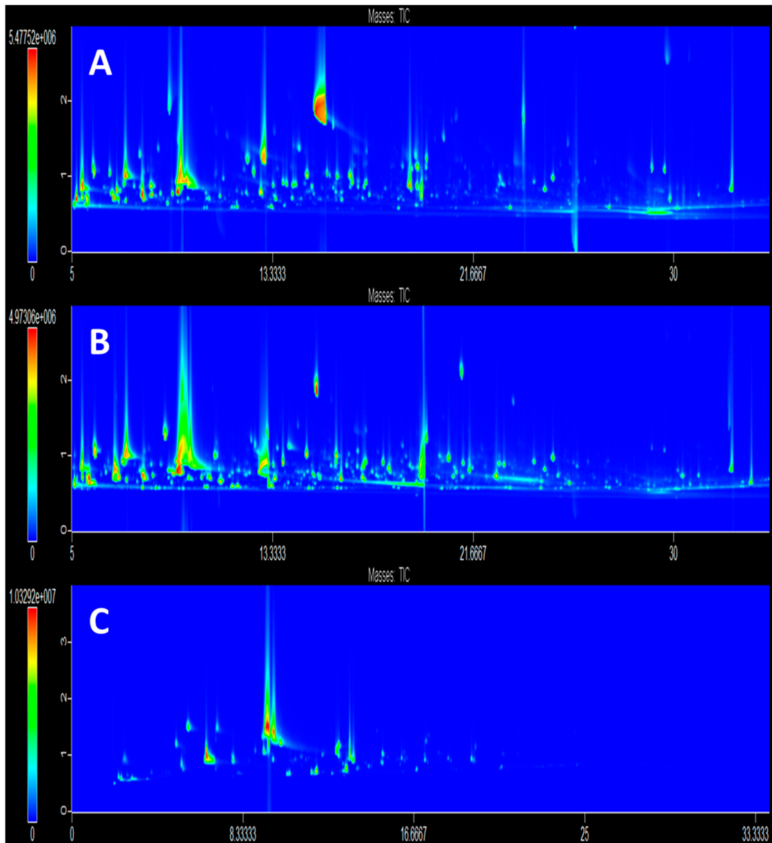
Figure 1. S. GCxGC-ToFMS chromatograms of fresh broccoli volatiles acquired using (A) – SAFE; (B) – SDE and (C) – SPME extraction techniques.
