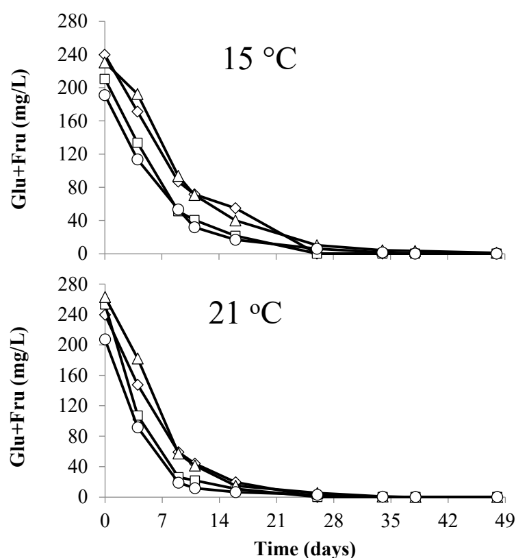
Figure 2. Changes in glucose and fructose during alcoholic fermentation at either 15 or 21 °C. Concurrent AF and MLF conducted by S. cerevisiae D47 and O. oeni Beta with pre-fermentation addition of T. delbrueckii Prelude™ (Δ); AF by S. cerevisiae D47 with pre-fermentation addition of T. delbrueckii Prelude™ (◊); AF by S. cerevisiae D47 (◻); concurrent AF and MLF conducted by S. cerevisiae D47 and O. oeni Beta (◐). Values are means from triplicate fermentations.
