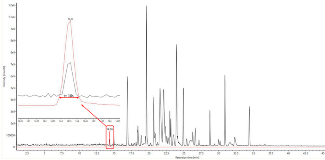
Figure 3. Overlay of Base Peak Intensity and Extracted Ion Chromatogram for narrowest peak corresponding to an identified peptide.
