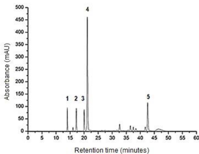
Figure S2. HPLC chromatogram of individual anthocyanin monoglucosides in Plavac Mali grape skin extract. The peaks correspond to: 1 delphinidin-3- O -glucoside, 2 cyanidin-3- O -glucoside, 3 petunidin-3- O -glucoside, 4 malvidin-3- O -glucoside, 5 peonidin-3- O -glucoside.
