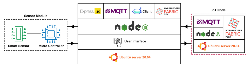
Figure 11. Application Node Architecture.
