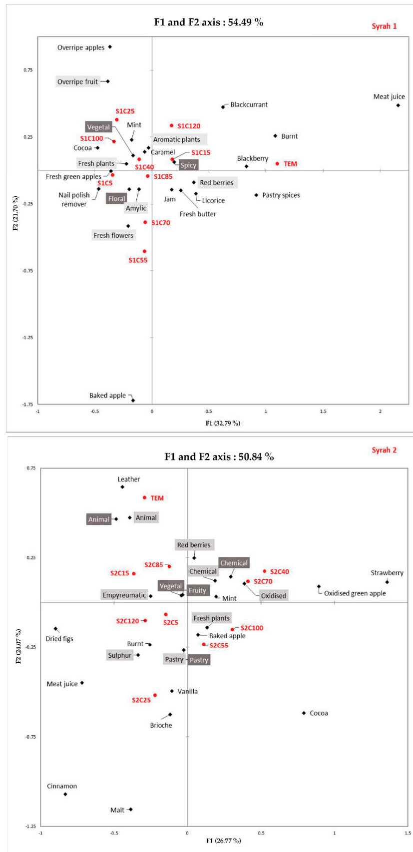
Figure 2. Correspondence analysis of HCATA results for each sample. SXCXY with X = the number of samples and Y = the corresponding spiked concentration. Families–Sub-families–olfactory terms. TEM = control wine without acetaldehyde addition.
