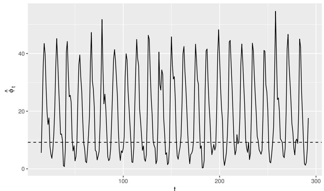
Figure 4. Estimated conditional precisions from the generalized BPSARMA model (solid line) and fixed precision estimate from the constant-precision BPSARMA model (dashed horizontal line); Manso reservoir inflow.
