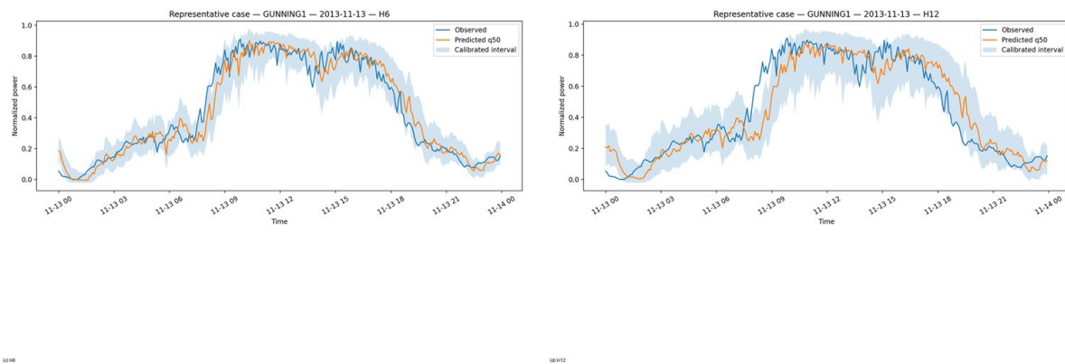
Figure 6. Daily forecasting illustration for a representative scenario on GUNNING1 (13 November 2013) at H1, H3, H6, and H12. (a) H1; (b) H3; (c) H6; (d) H12.
