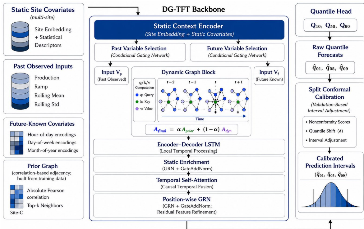
Figure 4. Architecture of the proposed DG-TFT-CQR model.
