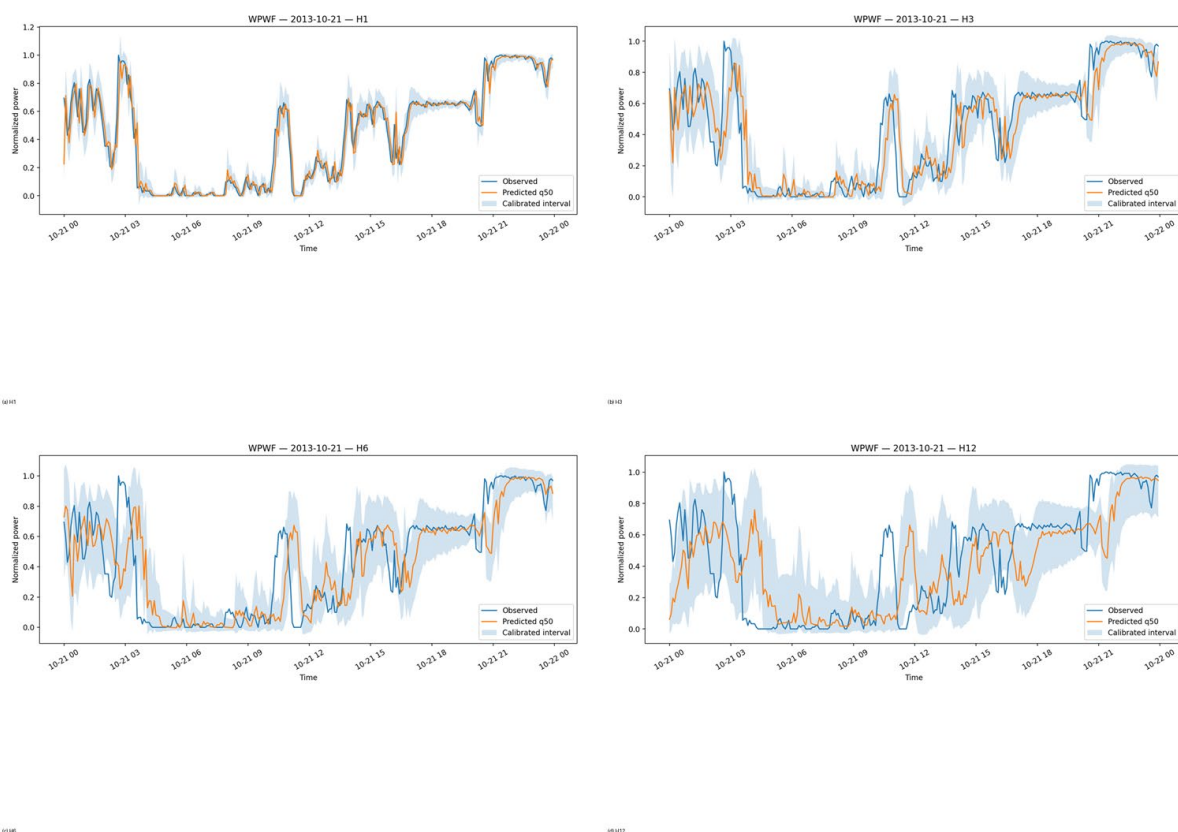
Figure 7. Daily forecasting illustration for a difficult scenario on WPWF (21 October 2013) at H1, H3, H6, and H12. (a) H1; (b) H3; (c) H6; (d) H12.
