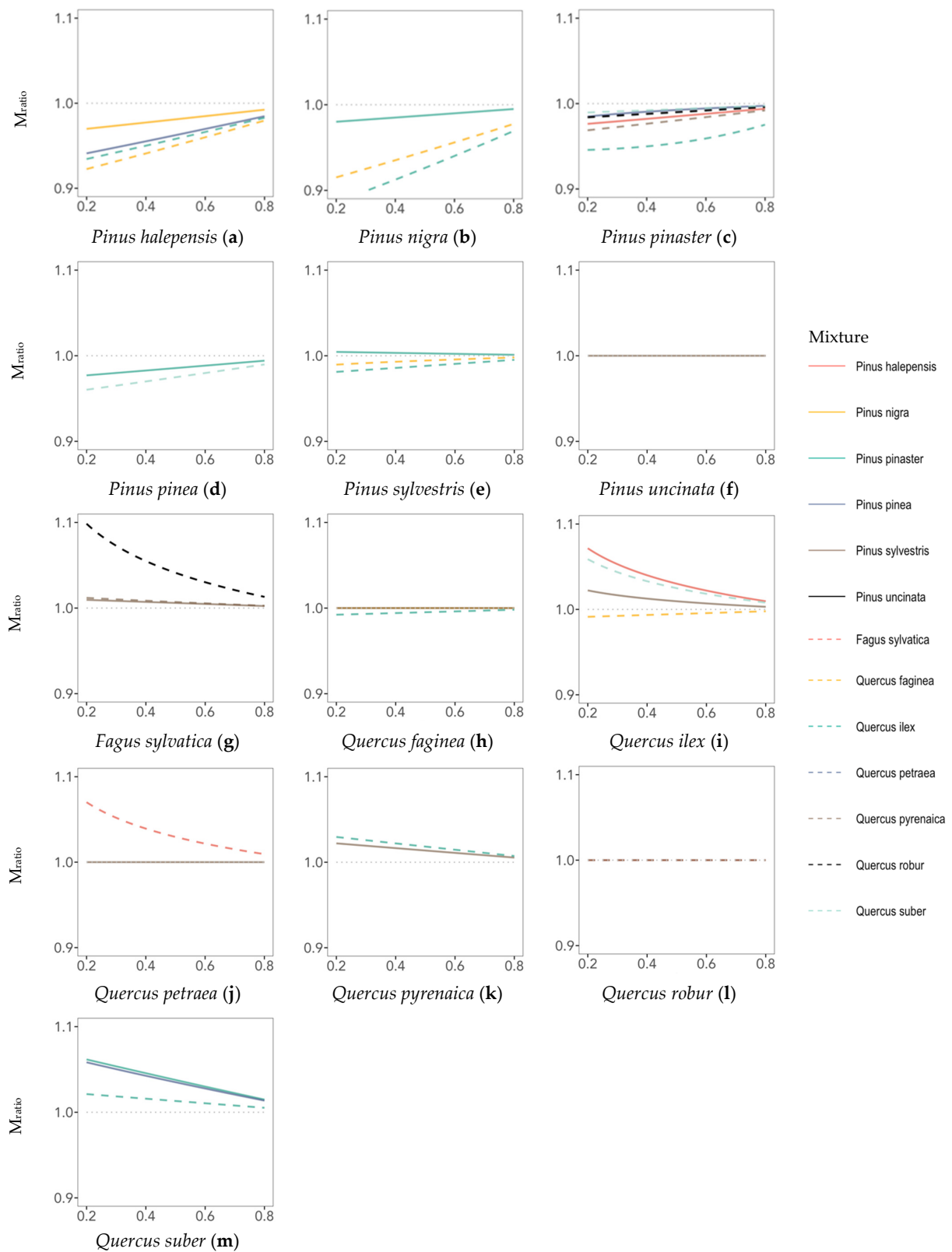
Figure 1. Variation of height under different species' mixing proportions ( m_1 -x-axis) based on the M_{ratio} (y-axis). Letters a-m indicate the species name in order to make reference to them along the text. Note: M_{ratio} represents whether height in mixed forests is higher ( M_{ratio} > 1 ) or lower ( M_{ratio} < 1 ) than pure stands. All independent variables (excepting m_1 ) have been fixed to the mean of each species.
