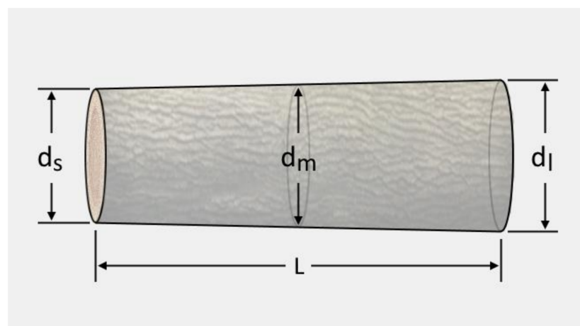
Figure 1. Scheme of determining parameters for the calculation of log volume.
