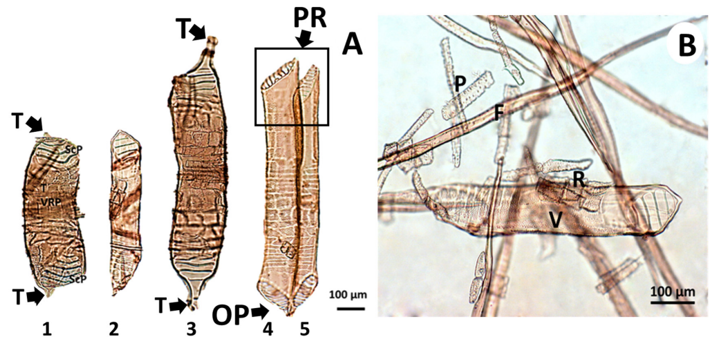
Figure 6. The compositions of cells in tapped S. sumatrana . (A) Vessel elements (1–5), tails of vessel element (T), parallel (PR) and opposite (OP) perforation plates between 4 and 5. (B) Fibers (F), parenchyma cell (P), vessel element (V), and ray (R). Scale bars: 100 \mu\text{m} .
