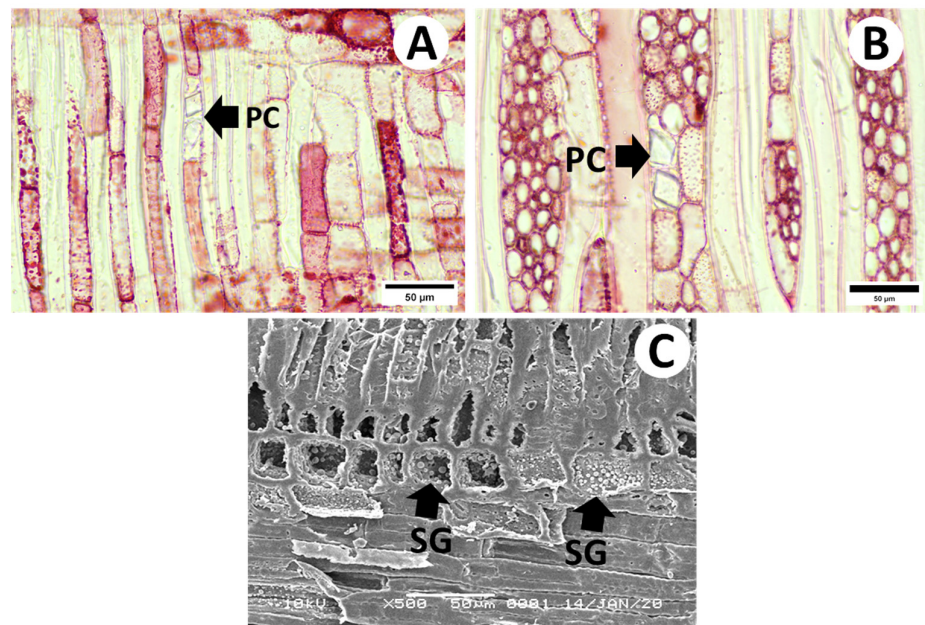
Figure 5. Oxalate prismatic crystals (PCs) in axial (A) and ray (B) parenchyma, as well as silica grain (SG) in ray parenchyma (C) of tapped S. sumatrana wood. Scale bars: 50 µm.
