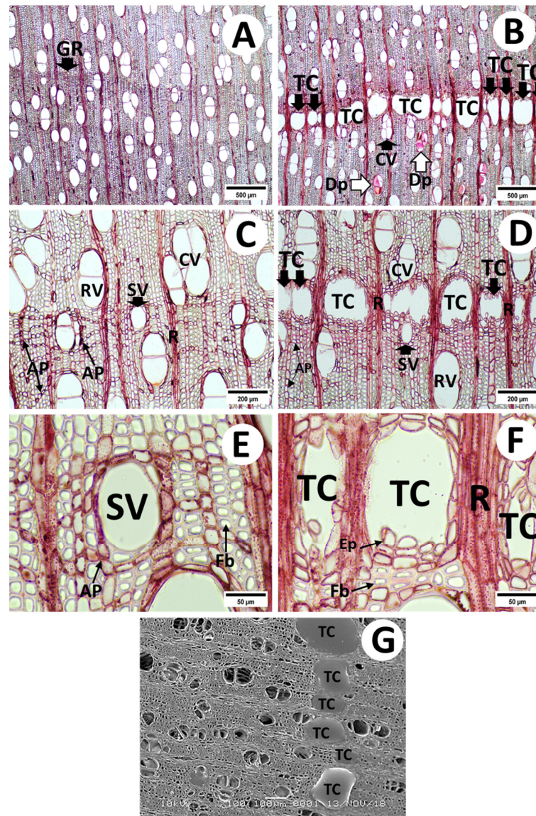
Figure 2. The optical (A–F) and scanning electron (G) micrographs of cross-sections of the untapped (A,C,E) and tapped (B,D,F,G) parts in tapped S. sumatrana . Growth ring (GR), traumatic resin canals (TCs), clustered vessels (CVs), radially arranged vessels (RVs), solitary vessels (SVs), deposits in vessels (Dp), rays (Rs), axial parenchyma (AP), fibers (Fb), and epithelial cells (Ep). Scale bars: 500 \mu\text{m} (A,B), 200 \mu\text{m} (C,D), 50 \mu\text{m} (E,F), and 100 \mu\text{m} (G).
