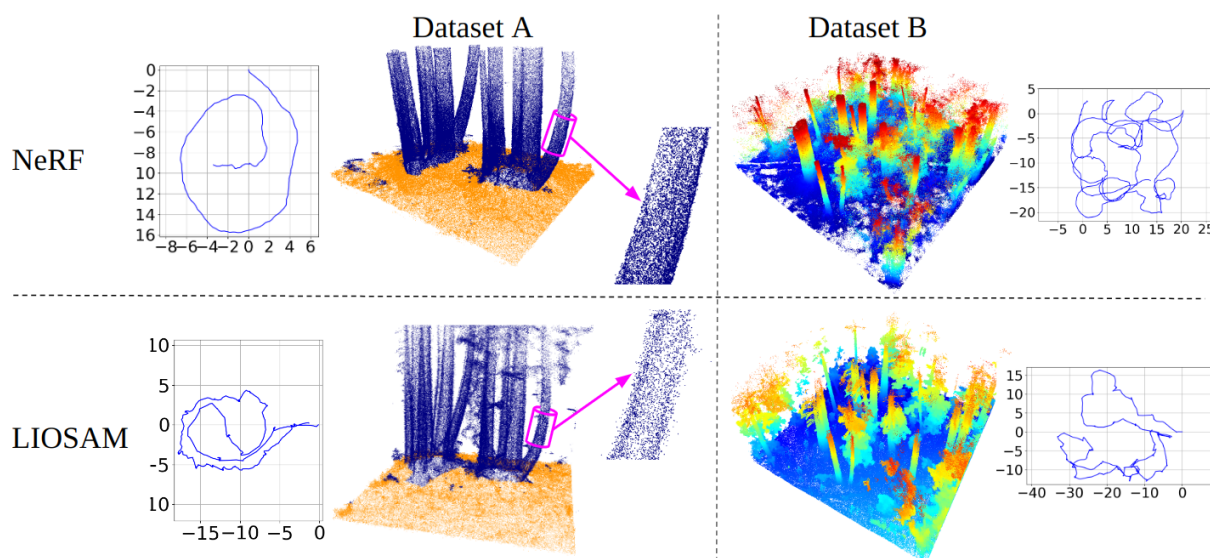
Figure 4. Forest reconstructions produced by SLAM ( bottom row) and NeRF ( top row) methods of both datasets. Adjacent plots are data collection trajectories for each reconstruction. In dataset A, we illustrate the effectiveness of segmentation between the ground points (orange) and trees (violet). We use a z-axis color gradient to enhance the visualization of dataset B reconstructions, as this region included more complex ground-level vegetation. The figure also compares a zoomed-in section of a tree trunk. The NeRF reconstruction is approximately 4× denser compared to SLAM, and is of higher surface quality.
