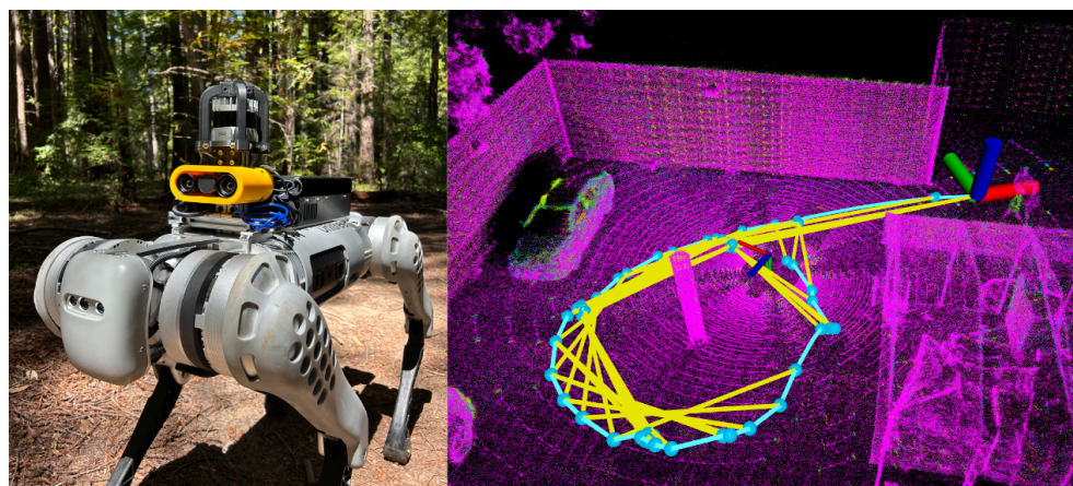
Figure 2. Quadruped robot creating a dense LiDAR-inertial reconstruction in a forest environment (left). LIOSAM visualization of estimated trajectory (torquoise), loop-closure events (yellow), and tightly aligned LiDAR scans (magenta) (right).
