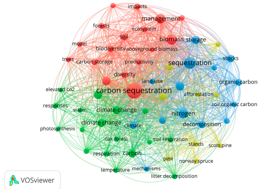
Figure 8. Keyword co-occurrence network showing major research themes related to oak forests and carbon sequestration. Node size indicates keyword frequency, while connections represent the thematic relationships among research topics.
