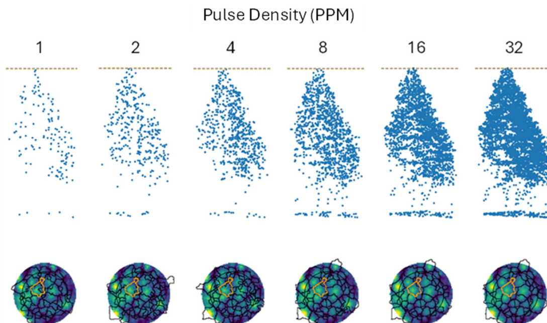
Figure 10. Visual change in point cloud density, definition of tree architecture, understory vegetation, and representation of ground surface resulting from increased pulse density.
