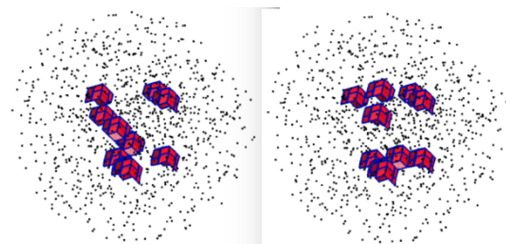
Figure 3. One 3DPT GoL oscillation pattern. The pattern is a oscillator period 2 and the two frames are shown.
