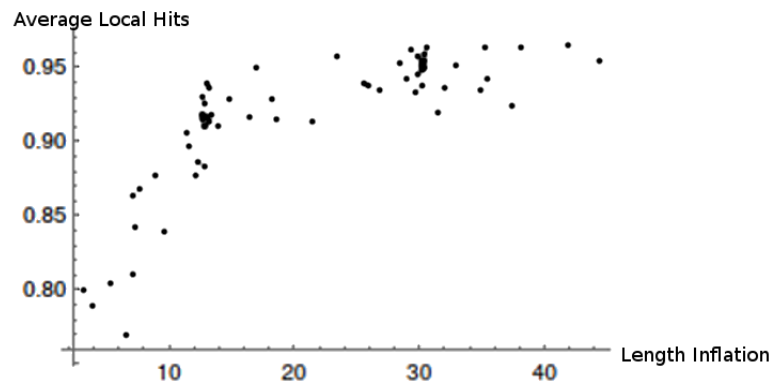
Figure 7. Average hits H_T(l) evolution under inflations.
