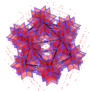
Figure 9. Central icosahedron oscillating pattern.
