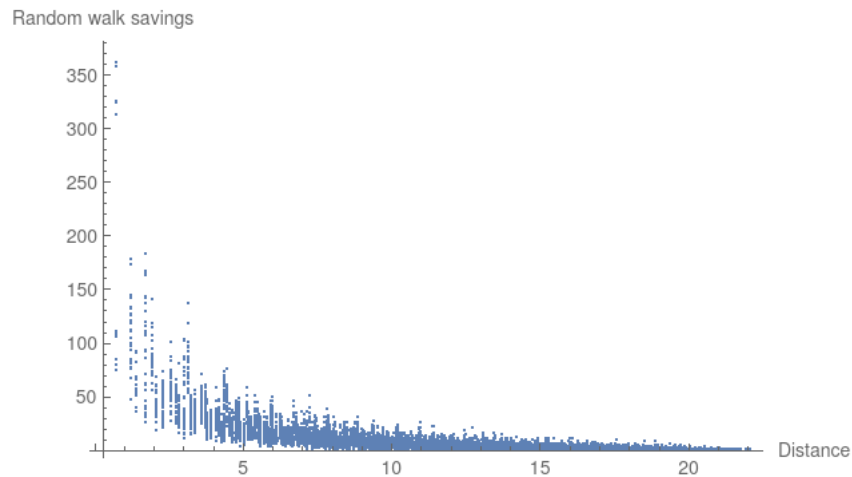
Figure 5. PRW hit potential.
